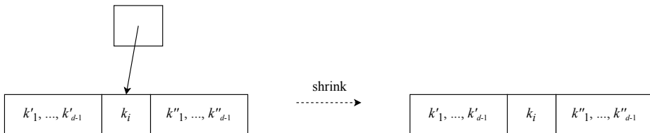
Figure 7.15: Shrink
