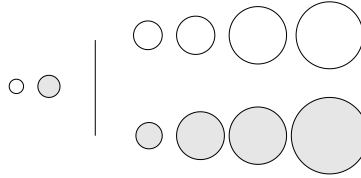
Figure 13.8: Merge
