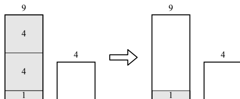
Figure 14.26: Fill the bigger jug, then pour to the smaller one twice.
