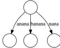
Figure C.1: The suffix tree for ‘banana’
