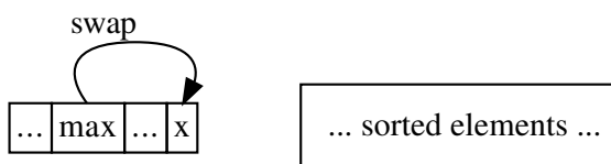
Figure 9.4: Select the maximum every time and put it to the end.
