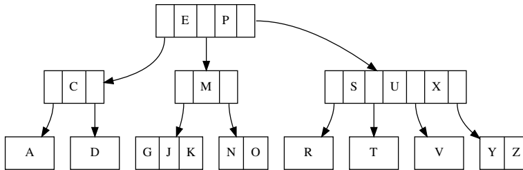
(a) 2-3-4 tree.
