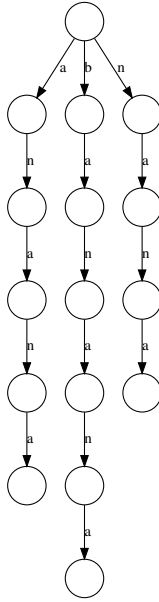
Figure C.3: Suffix trie for 'banana'
