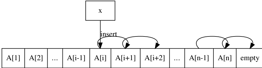
Figure 3.3: Insert x to array A at position i .
