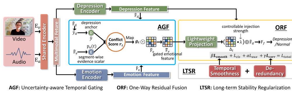
Fig. 3 Overall framework of A2F-Net: shared audio–visual encoding produces multimodal features; anchor-guided uncertainty-aware temporal gating (AGF, Sec. 3.3) suppresses emotion segments conflicting with the depression anchor; one-way residual fusion (ORF, Sec. 3.4) injects reliable emotional increments into the depression representation; long-term stability regularization (LTSR, Sec. 3.5) with temporal smoothness and de-redundancy constraints further improves robustness for binary depression detection.
