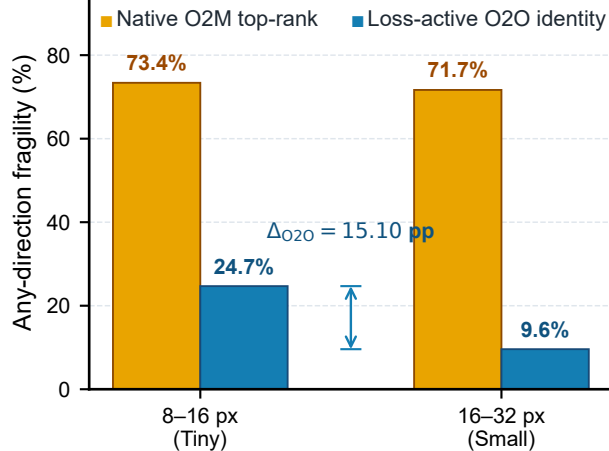
(c) Margin \rightarrow identity fragility
