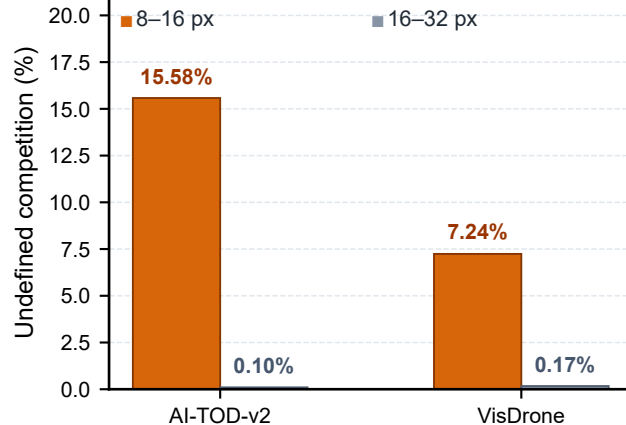
(b) Undefined-competition boundary
