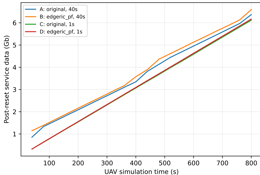
contention_hover | seed 0 | paired trajectories | aligned post-reset metrics
