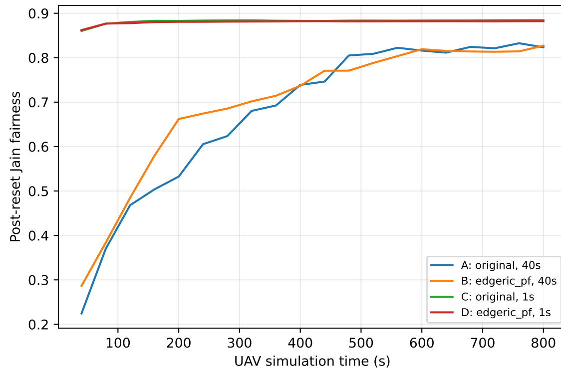
contention_hover | seed 0 | paired trajectories | aligned post-reset metrics
