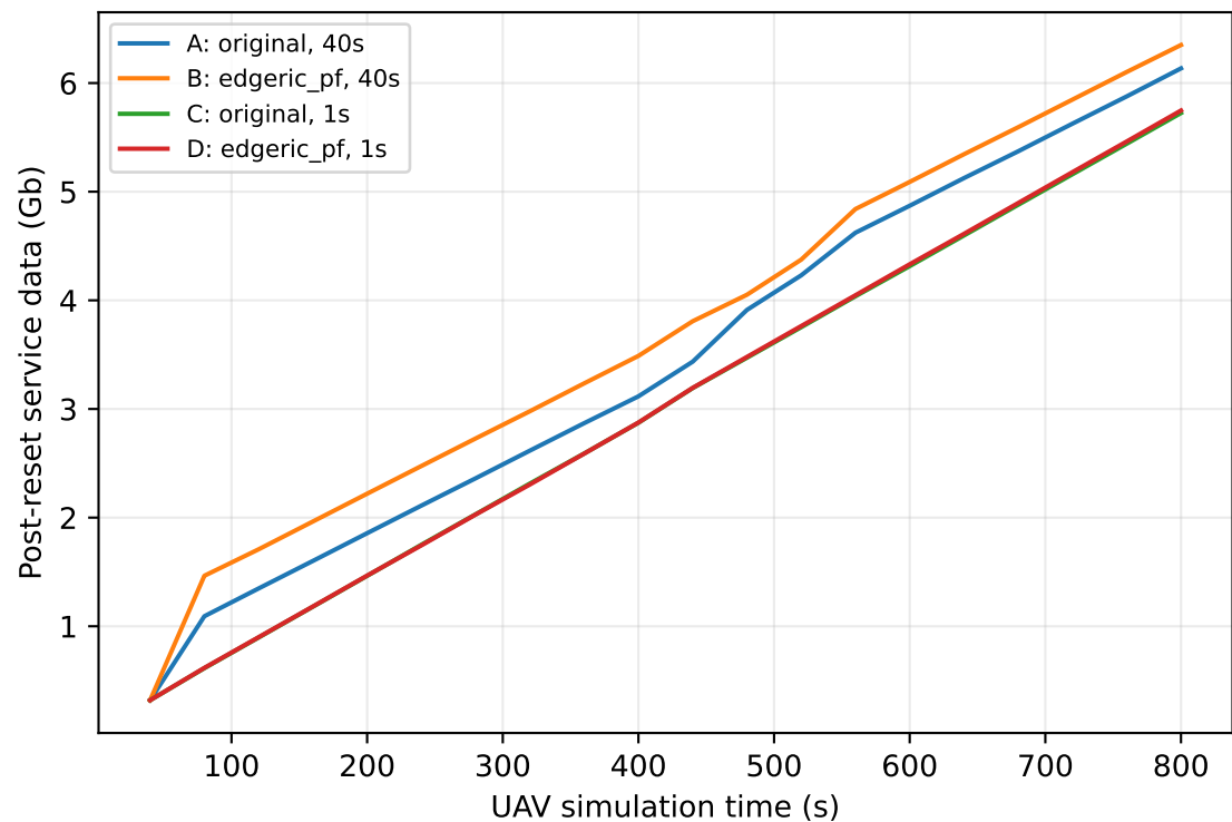
contention_motion | seed 0 | paired trajectories | aligned post-reset metrics
