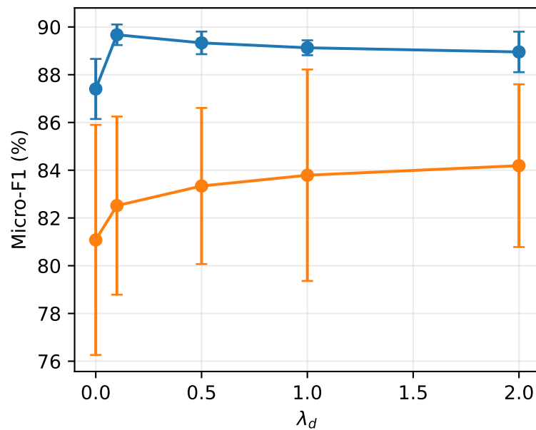
DVCL hyperparameter sensitivity on DBLP
