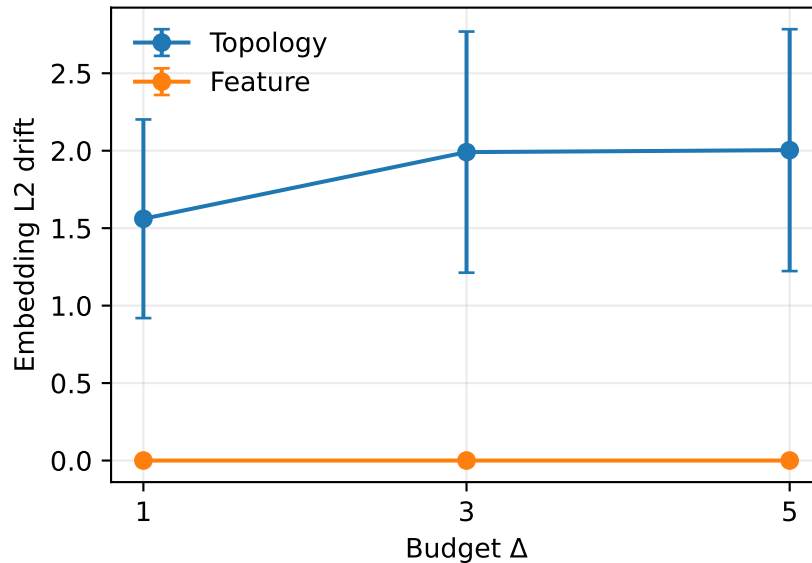
View representation drift
