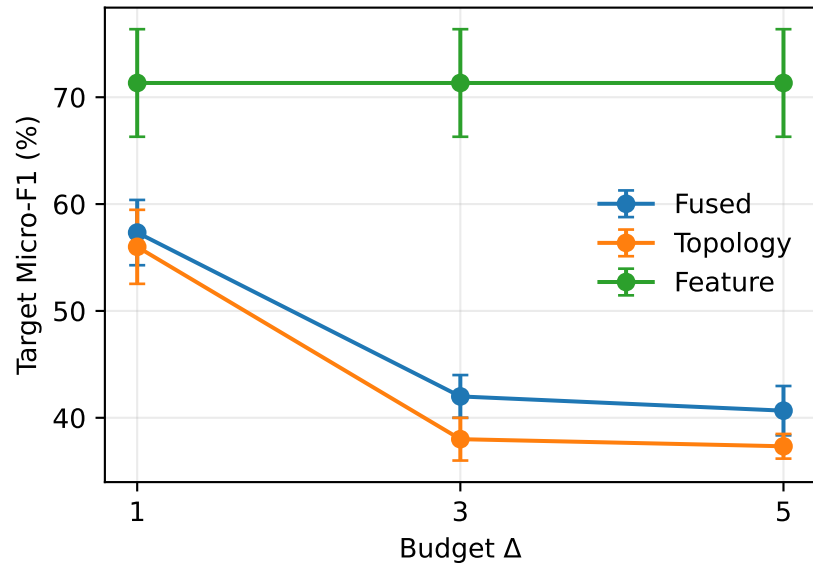
Branch performance
