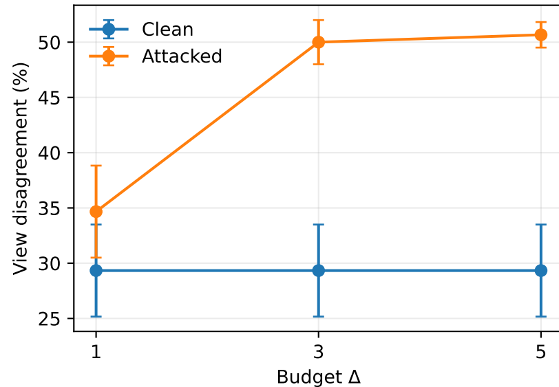
Prediction disagreement
