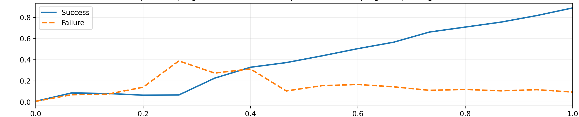
Jev-1.13 progress (state)* — raw expected absolute progress, privileged state
