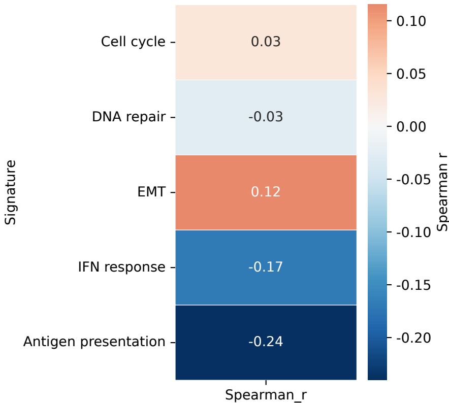
Correlation with RLP3/RLP4 combined score
