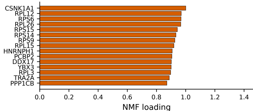
RLP1: top 15 loading regulators
