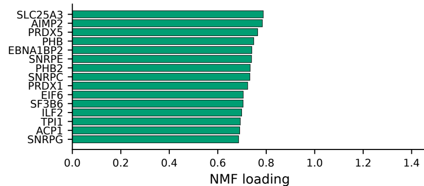
RLP4: top 15 loading regulators
