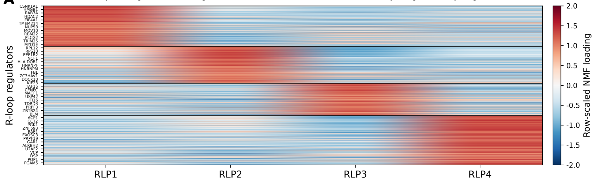
Complete gene-loading matrix of four NMF-derived R-loop regulator programs
