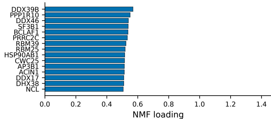
RLP3: top 15 loading regulators
