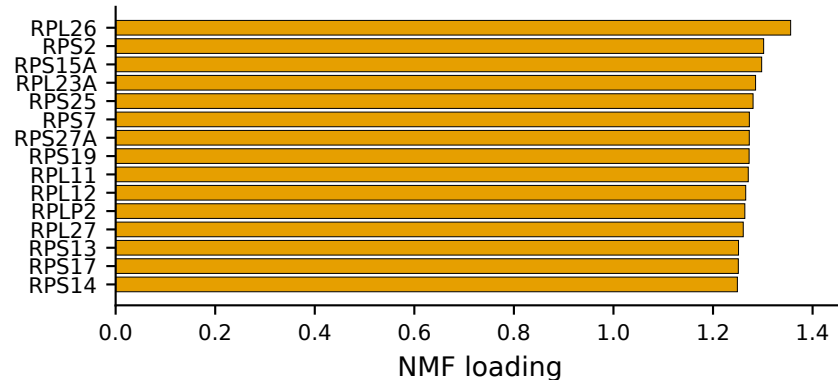
RLP2: top 15 loading regulators
