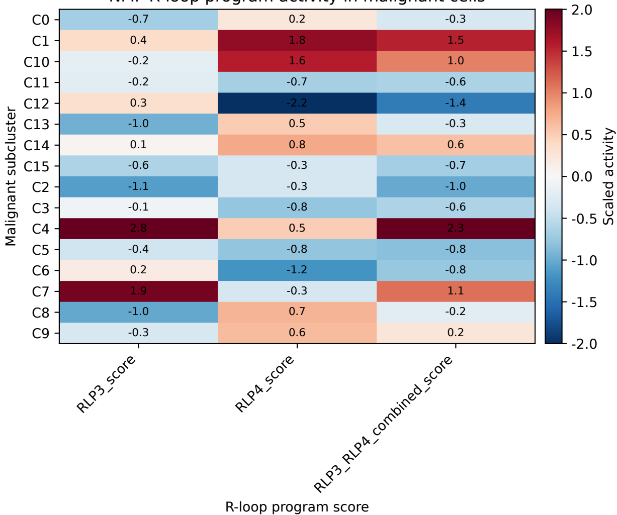
NMF R-loop program activity in malignant cells
