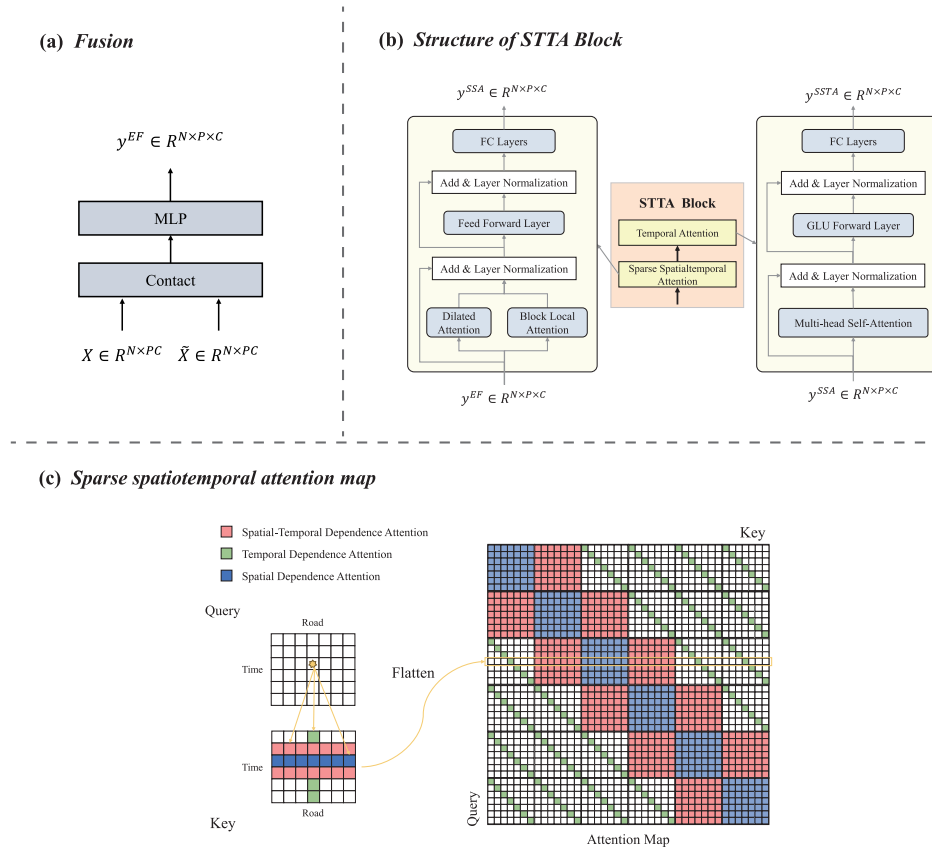
Fig. 2. Overall architecture of the spatial-temporal feature enhancement network framework. (a) Fusion , used to fuse global low-rank priors and observation data; (b) Structure of STTA Block , which consists of sparse spatiotemporal attention (left) and temporal attention (right). The sparse spatiotemporal attention mechanism consists of two attention modules: dilated attention and block local attention, which focus on the elements on the diagonal and block diagonal, respectively; (c) Sparse spatiotemporal attention map , which serves as the core building blocks for SSA. Enable attention mechanisms to focus only on certain elements to establish effective spatiotemporal relationships and reduce redundant information. Blue represents spatial dependence, green represents temporal dependence, and red indicates spatial-temporal dependence.
