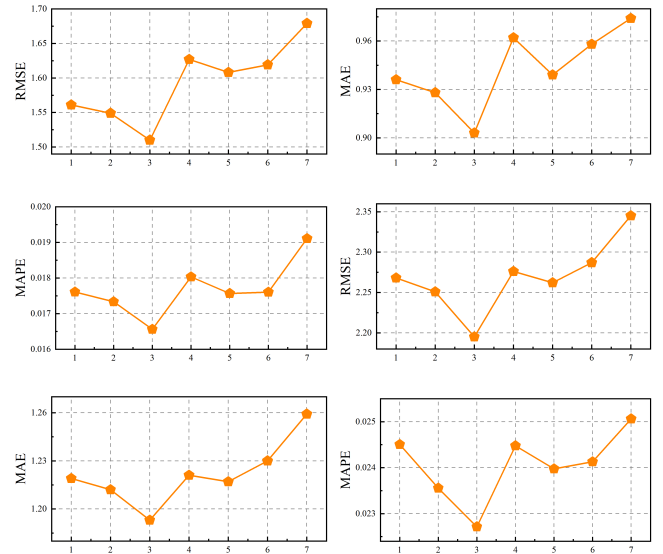
Fig. 10. Imputation accuracy at 30% and 70% random missing scenarios for different spatial-temporal attention scope l .
