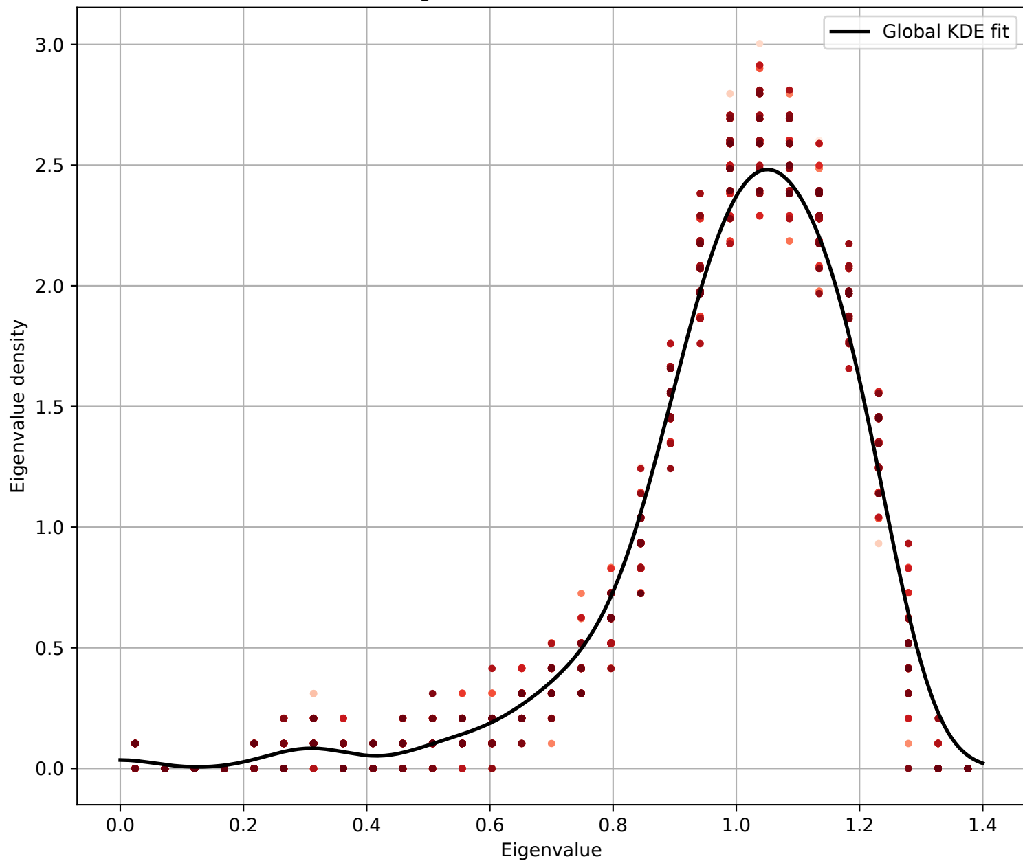
Binned eigenvalue distribution with KDE fit
