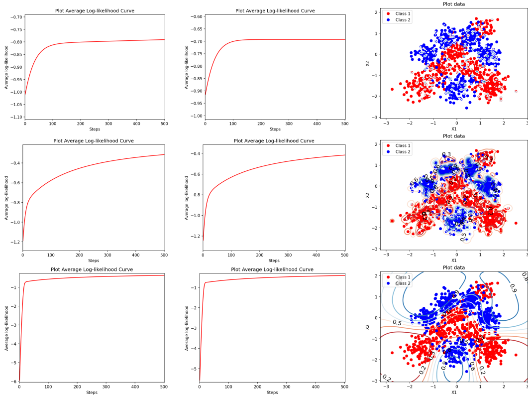
Figure 4: Train log-likelihood (left), test log-likelihood (middle), and predictive contours (right). Top row: l = 0.01 , \eta = 0.0001 , T = 500 . Middle row: l = 0.1 , \eta = 0.0005 , T = 500 . Bottom row: l = 1.0 , \eta = 0.0001 , T = 500 . All T = 500 .
