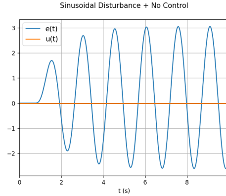
Figure 8: Sinusoidal + no control.
