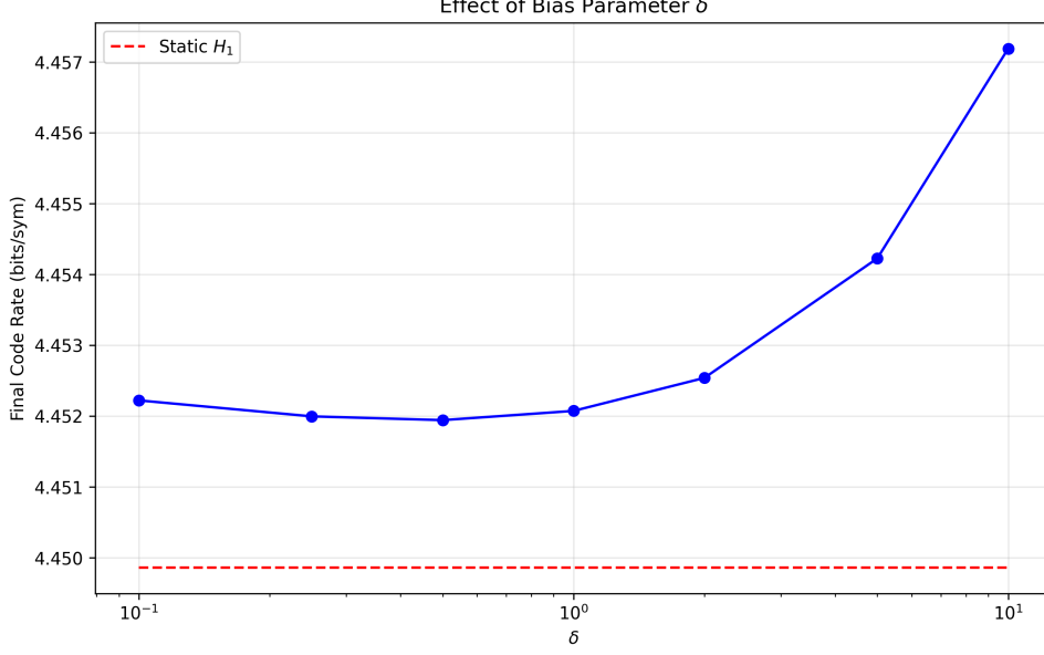
Figure 4: Effect of bias \delta on the final compression rate, measured on the entire Hamlet text ( N \approx 207k ). The minimum occurs at \delta \approx 0.5 (Krichevsky-Trofimov estimator).
