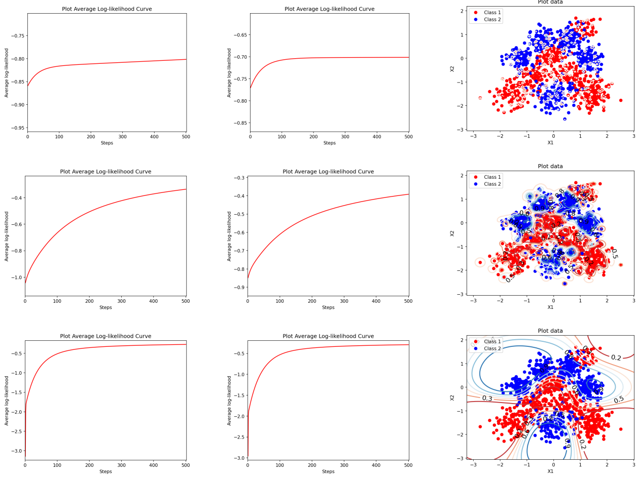
Figure 4: Training log-likelihood (left), test log-likelihood (middle), and predictive probability contours (right) for the RBF-expanded logistic classifier. Top row: l = 0.01, \eta = 0.0001, T = 500 . Middle row: l = 0.1, \eta = 0.0005, T = 500 . Bottom row: l = 1.0, \eta = 0.0001, T = 500 .
