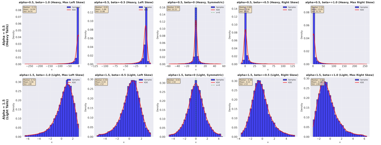
Figure 9: Alpha-stable distributions for \alpha = 0.5 (top, heavy tails) and \alpha = 1.5 (bottom, lighter tails) with varying \beta (skewness). Heavy-tailed distributions ( \alpha = 0.5 ) produce extreme outliers requiring plot clipping.
