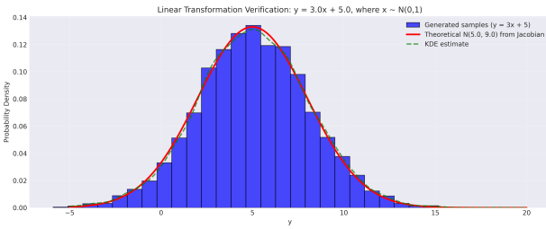
Figure 5: Verification of linear transformation y = 3x + 5 where x \sim \mathcal{N}(0, 1) . The histogram matches theoretical \mathcal{N}(5, 9) .
