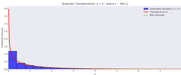
Figure 6: Verification of quadratic transformation y = x^2 . Sample mean \approx 1.0 and variance \approx 2.0 match theoretical \chi_1^2 moments.
