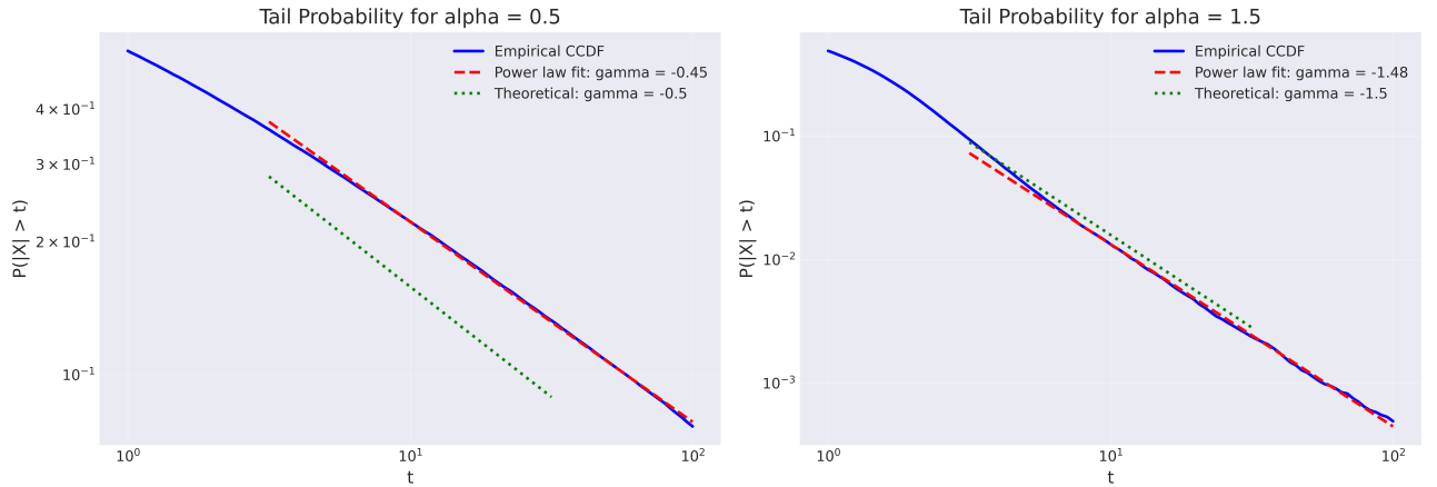
Figure 10: Power law tail fitting for \alpha -stable distributions. Log-log plots of P(|X| > t) versus t show linear decay with slope \gamma \approx -\alpha , confirming the theoretical prediction.
