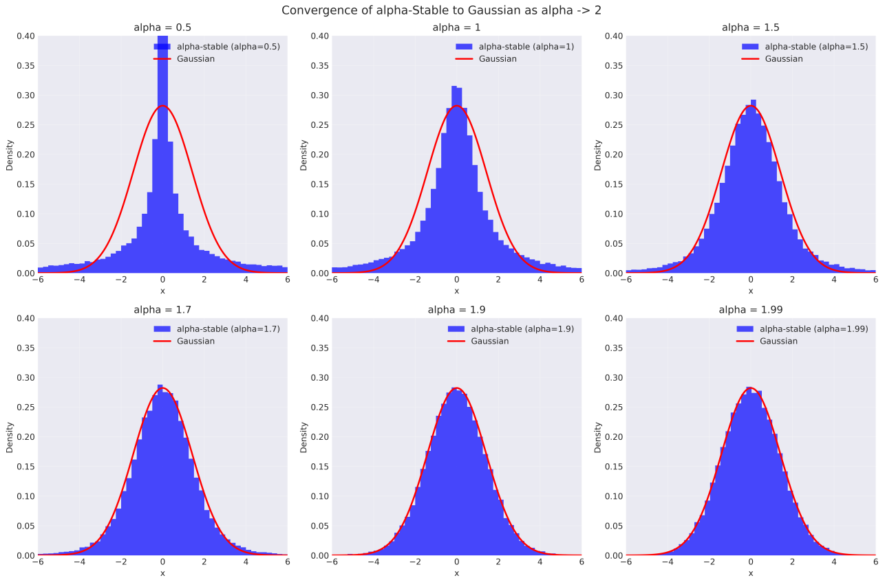
Figure 11: Convergence of \alpha -stable to Gaussian as \alpha \rightarrow 2 . For \alpha = 0.5 , the distribution has extremely heavy tails. As \alpha increases through 1.5, 1.7, 1.9, 1.99, the distribution progressively approaches the Gaussian (red curve).
