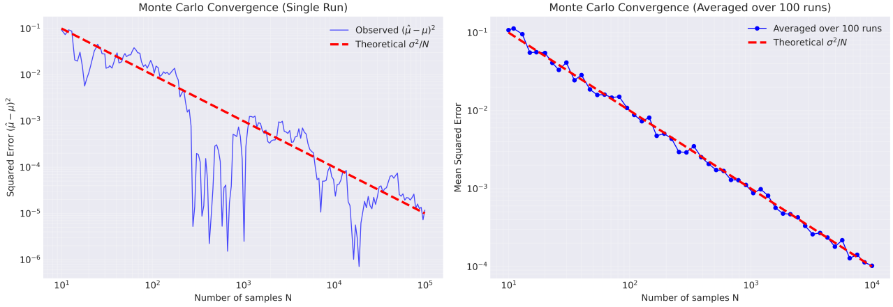
Figure 8: Monte Carlo convergence for exponential distribution. Left: Single run showing squared error (\hat{\mu} - \mu)^2 versus N with theoretical variance \sigma^2/N (dashed). Right: Averaged squared error over 100 runs confirms 1/N decay rate.
