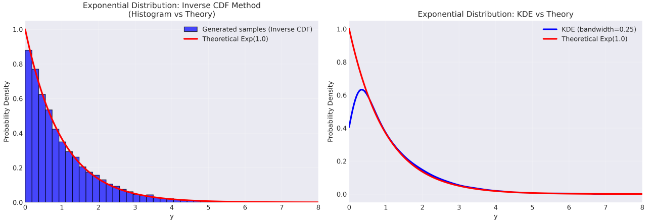
Figure 7: Exponential distribution via inverse CDF method. Histogram (left) matches theoretical PDF. KDE (right) shows boundary effects: peak underestimated ( \approx 0.65 vs 1.0 ) due to Gaussian kernels extending into y < 0 .
