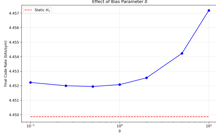
Figure 4: Effect of bias \delta on the final compression rate, measured on the entire Hamlet text ( N \approx 207k )
