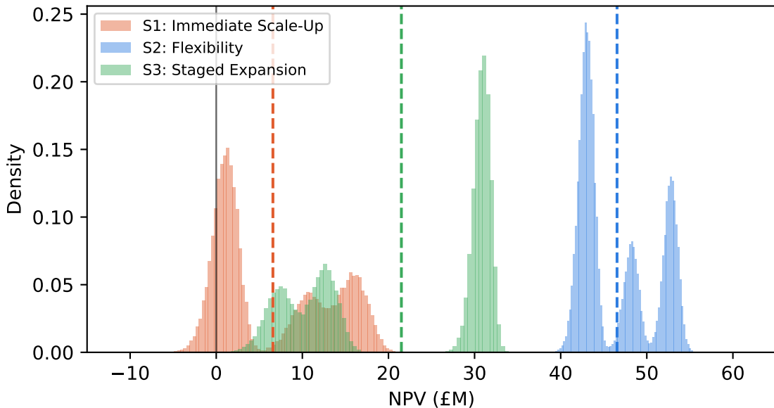
NPV Distribution (dashed = E[\text{NPV}] )
