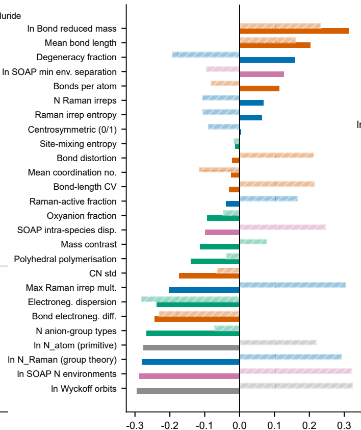
(b) X loadings (solid: LV1; hatched: LV2)
