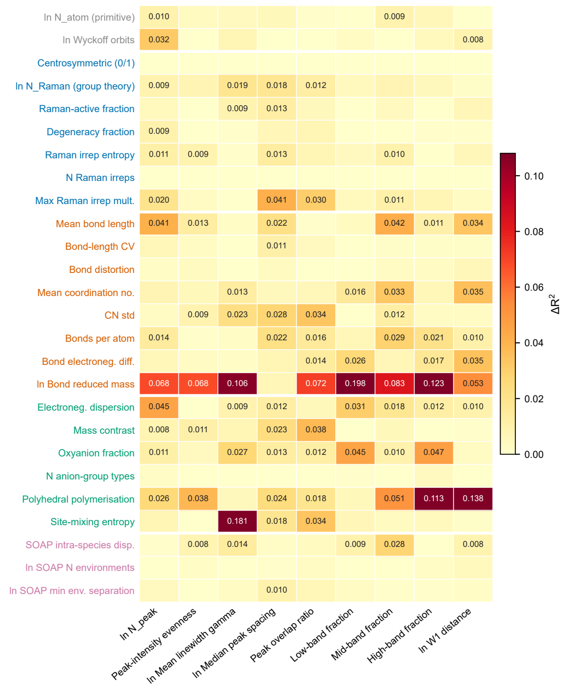
(a) Single-feature permutation importance ( \Delta R^2 , held-out folds)
