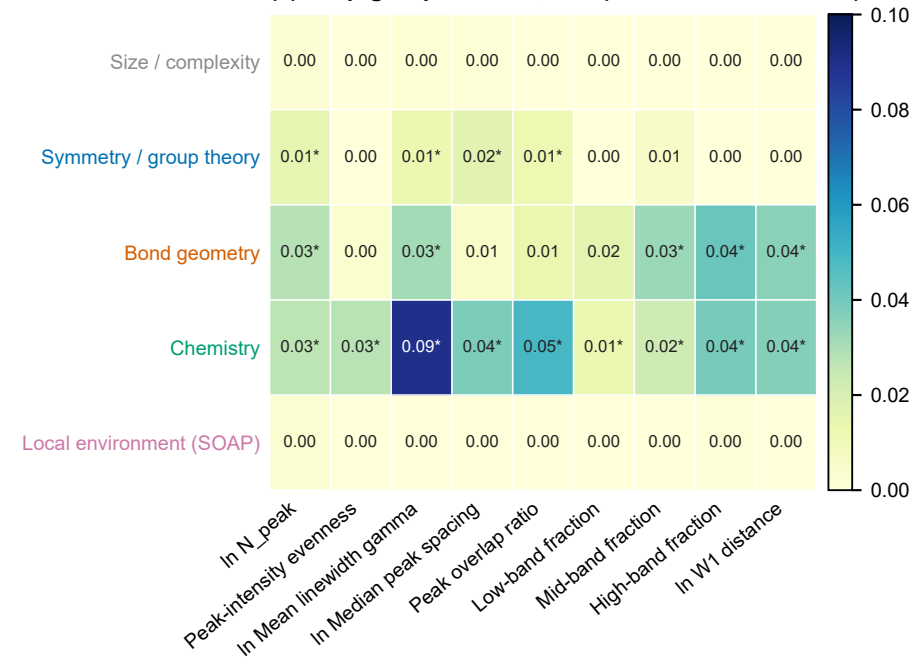
(c) Drop-group ablation, \Delta R^2 (* = 95% CI excludes 0)
