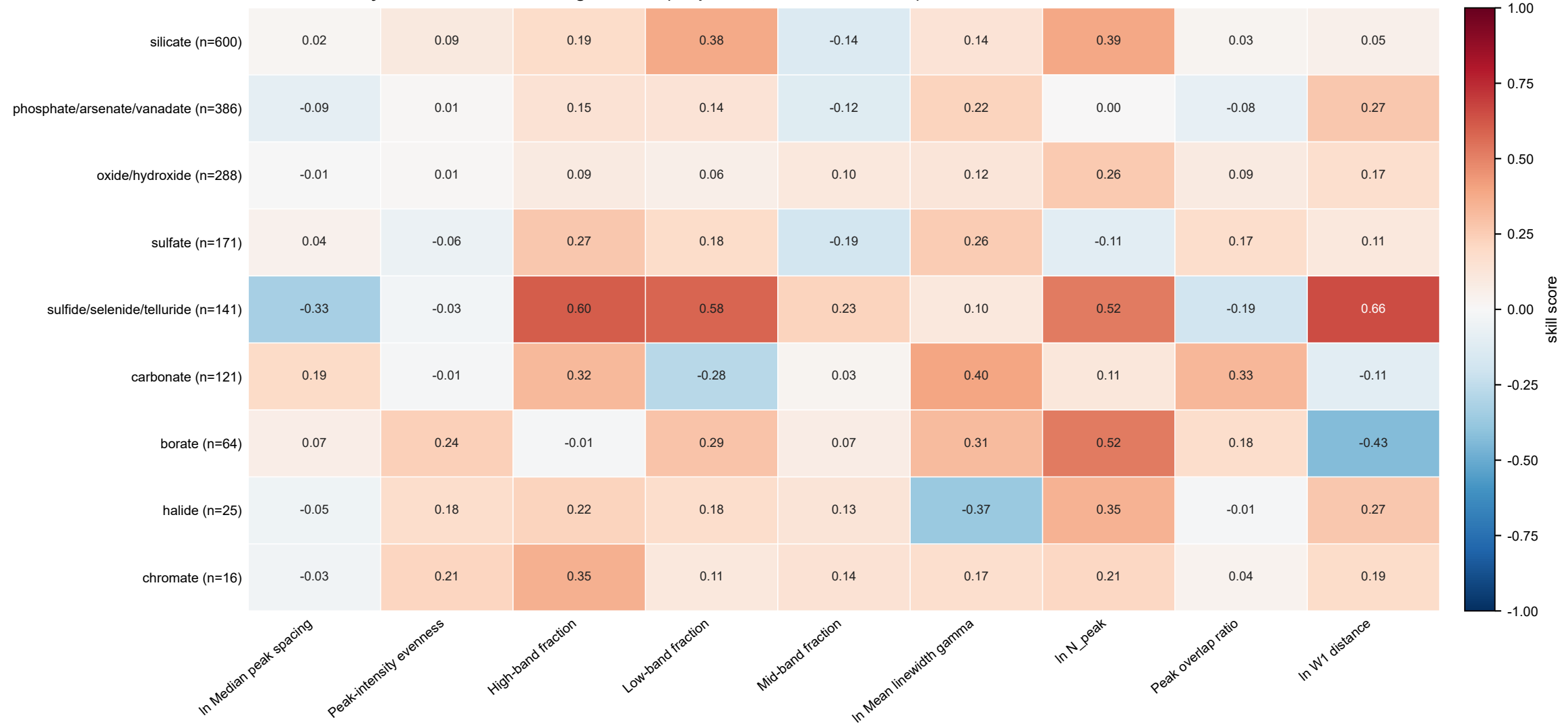
Leave-one-family-out skill score vs. training-set mean (1 = perfect, <0 worse than mean)
