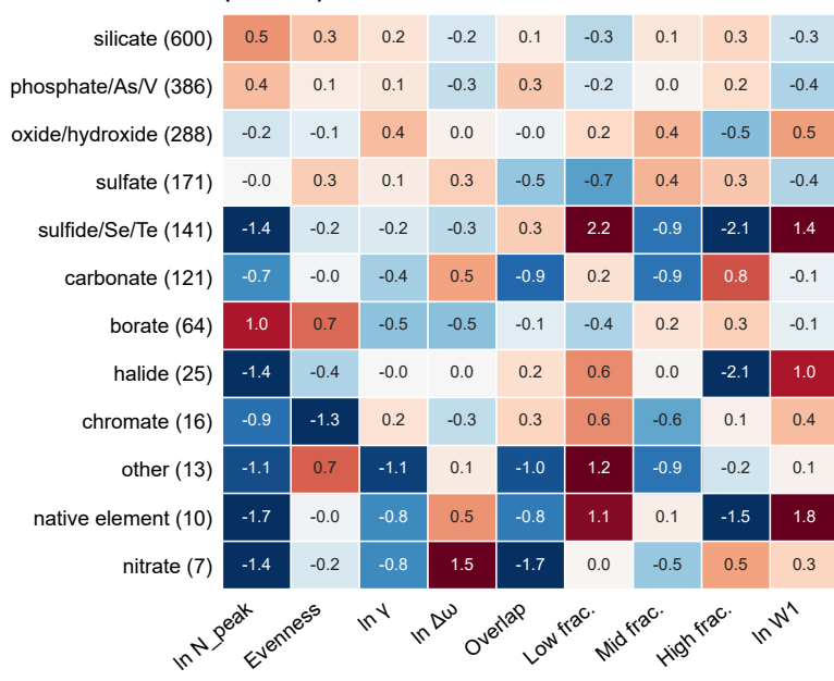
(c) Median spectral profile (z-score)
