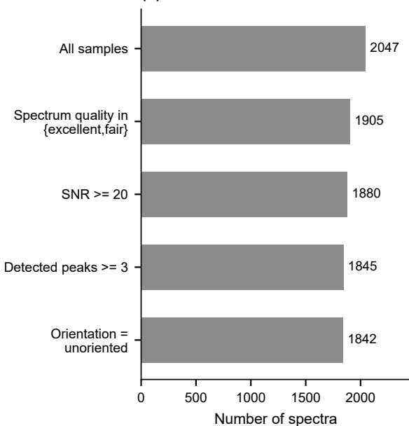
(b) QC funnel
