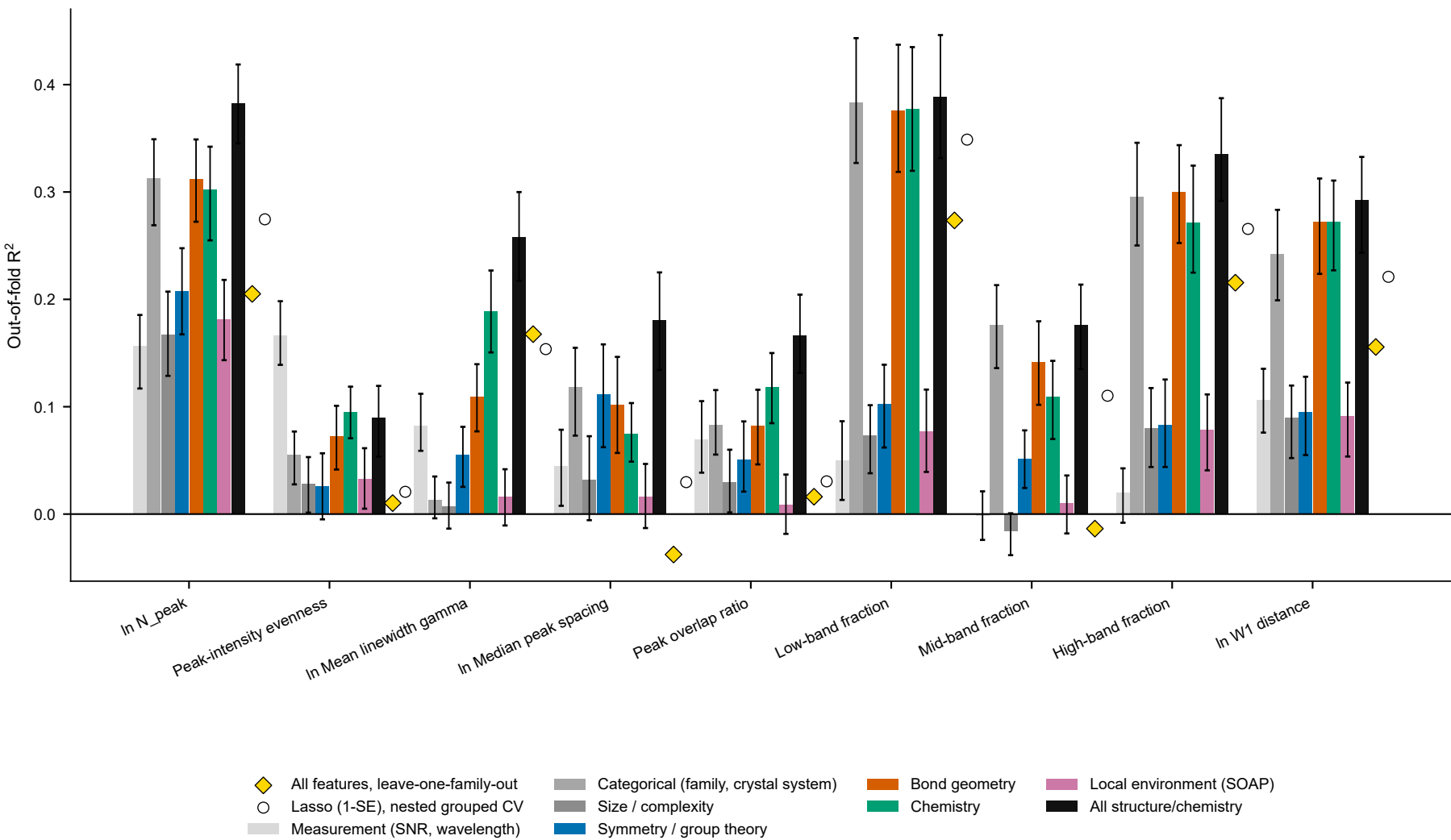
Predictive power of structural/chemical descriptors (bars: grouped CV by formula, 95% cluster-bootstrap CI)
