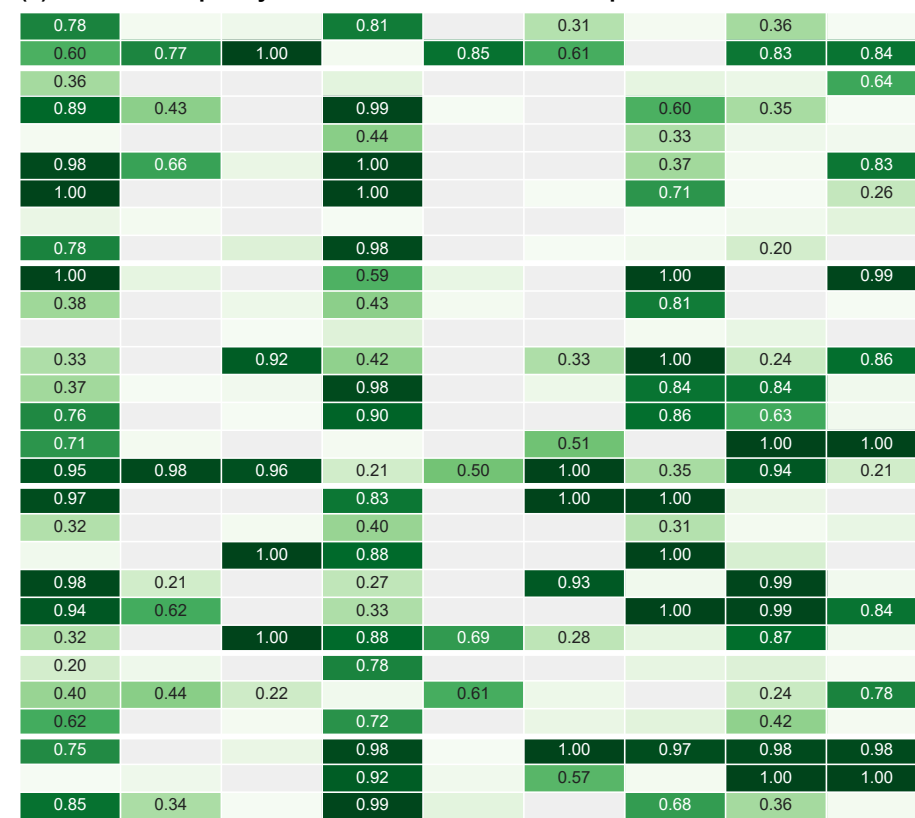
(b) Selection frequency in 100 formula-cluster bootstraps
