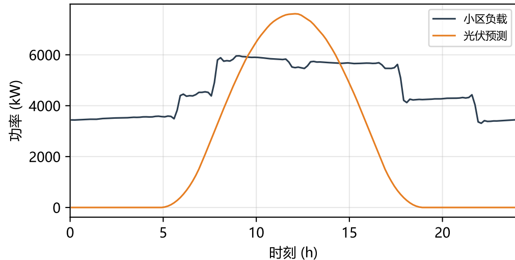
(b) 负载与光伏
