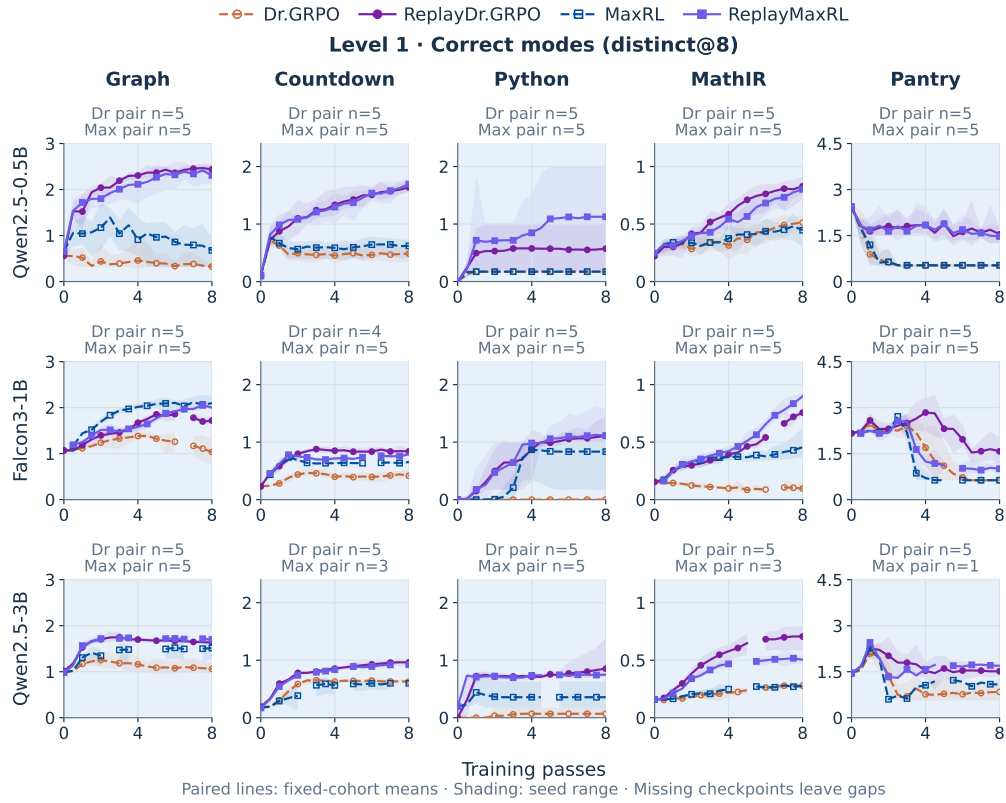
Figure 11: Verified modes throughout training at all three model scales. The same model rows, methods, seeds, and checkpoints as Figure 10, now measuring distinct@8 . Lines are descriptive fixed-cohort means and bands show seed ranges. A count of one has no band. Domain-specific vertical scales are shared across model rows; absolute heights across different domains should be read against their labeled axes. Missing evaluations are never carried forward or joined across a gap.
