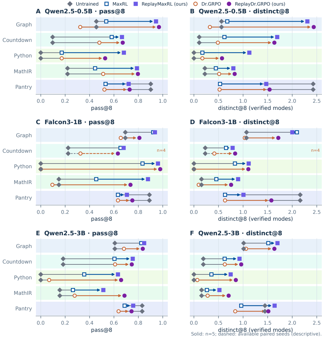
Figure 10: Per-domain results behind the cross-domain averages in Figure 5. Rows show Qwen2.5-0.5B, Falcon3-1B, and Qwen2.5-3B; columns show correctness and raw support. MaxRL–ReplayMaxRL pairs retain five terminal seeds throughout the two smaller models and Qwen2.5-3B: every MaxRL domain uses n = 5 . Solid connectors identify these complete comparisons. Dr.GRPO–ReplayDr.GRPO uses four admissible seeds for Falcon Countdown and five elsewhere. Domain tints match Figure 2. Replay arrows, trained-arm markers, and untrained references use the same encoding as Figure 5. The E118 model index groups the archived exports by model and domain.
