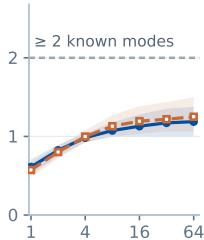
Python factors
