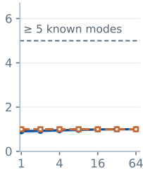
MathIR
