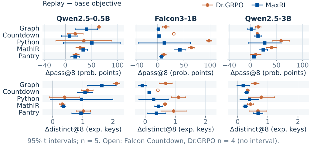
Figure 8: Replay effects on full-test success and sampled breadth. Terminal replay-minus-control contrasts hold Dr.GRPO or MaxRL fixed across all five domains and three scales. Every MaxRL cell has five paired seeds; one Dr.GRPO cell has four. Domain averages use shared seeds. These outcomes use all held-out prompts, unlike collision’s eligible populations. Appendix G.2 retains exact cohorts and intervals.
