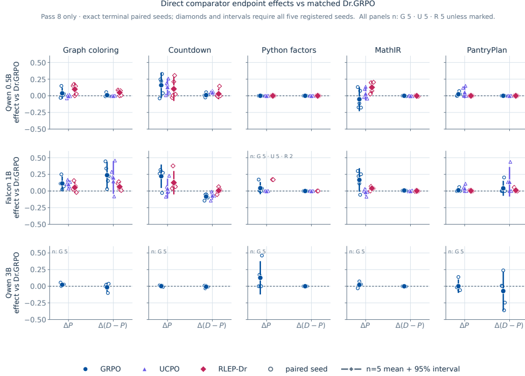
Figure 14: Direct alternatives produce local rather than uniform final gains. Each effect subtracts the same-seed Dr.GRPO control from the comparator after eight passes. Effects are shown for pass@8 and extra verified modes beyond the first success. Circles are paired seeds; diamonds and 95% Student- t intervals appear only for complete five-seed blocks. Exact n is printed, and unsupported comparisons remain blank rather than being extrapolated or imputed at any seed.
