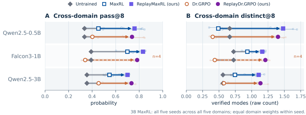
Figure 5: MaxRL and replay at all three model scales. Tracks connect initial, trained, and replay models. Complete tracks average within seed. All MaxRL tracks use five paired seeds in every domain, including 3B; Falcon Dr.GRPO uses four common seeds. Archived models.
