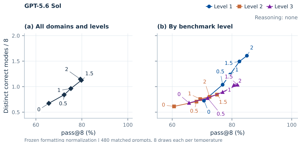
Figure 21: Temperature traces pass@8 and verified breadth. GPT-5.6 Sol, with 480 fixed prompts and eight draws each at T \in \{0, 0.5, 1, 1.5, 2\} . Left: all domains and levels; right: separate levels, averaging five domains equally. Empirical pass@8 is the fraction with at least one correct draw; distinct@8 averages unique correct modes, including zeroes. Connected points use reasoning none and the frozen formatting normalizer. Appendix J.3 gives pointwise uncertainty intervals for every benchmark level and all five measured temperatures.
