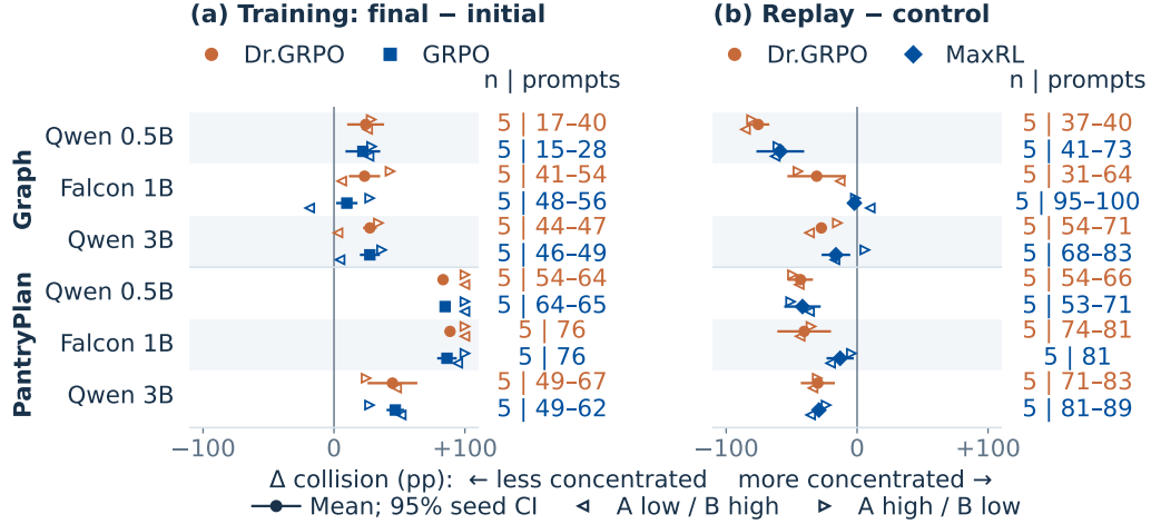
Figure 18: Training concentrates correct outputs; replay can reduce concentration. Graph/PantryPlan at three scales. Baselines compare final versus own initial outputs; replay compares matched terminal arms with the fresh objective fixed. Primary and disjoint-stream estimates retain separate eligible populations. Intervals describe five measured seed means; coverage and exceptions: Appendix H.1.
