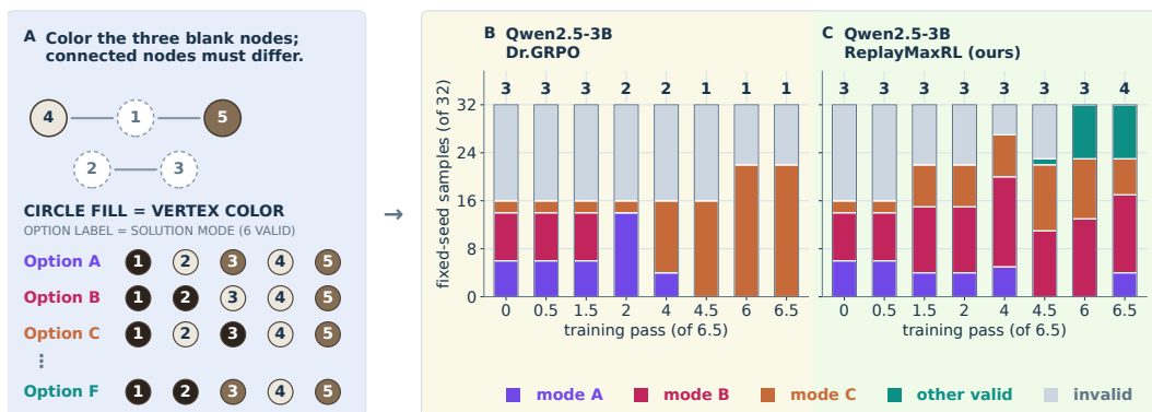
Figure 1: Correctness can rise while sampled alternatives narrow. One graph admits six valid colorings. Bars pool four saved eight-sample groups from matched Qwen2.5-3B runs. At pass 6.5, Dr.GRPO produces 22/32 correct from one mode; ReplayMaxRL produces 32/32 across four. This illustration changes both the fresh objective and replay; Figure 5 separates them.
