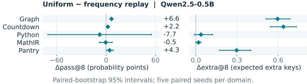
Figure 17: Uniform versus frequency-weighted replay. Paired Qwen2.5-0.5B contrasts show pass@8 and extra modes in each domain; the text reports the equal-domain mean. Intervals use paired-seed bootstrap with five seeds. The mean resamples whole seed vectors. Uniform weighting increases average extra modes, while its average correctness effect remains uncertain.
