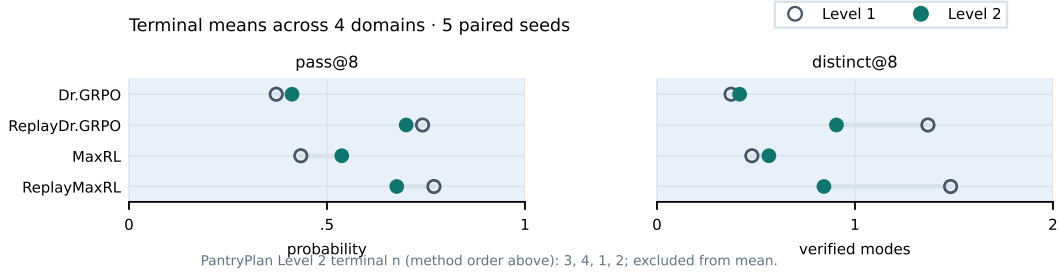
Figure 6: Replay across difficulty levels with Qwen2.5-0.5B-Instruct. Open/filled markers: Level 1/2. Means weight four complete domains equally within five paired seeds shared by both levels and all methods. Pantry remains separate (Appendix G.3). Archived models.
