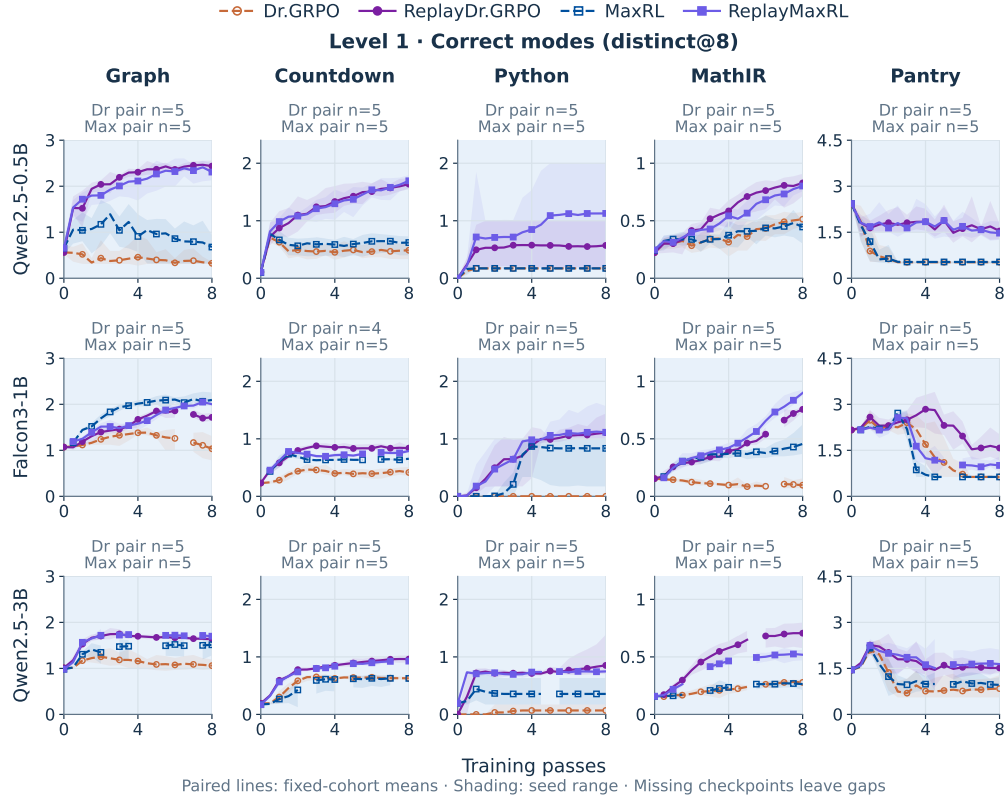
Figure 12: Verified modes throughout training at all three model scales. The same model rows, methods, seeds, and checkpoints as Figure 11, now measuring distinct@8. Lines are descriptive fixed-cohort means and bands show seed ranges. A count of one has no band. Domain-specific vertical scales are shared across model rows; absolute heights across different domains should be read against their labeled axes. Missing evaluations are never carried forward or joined across a gap.
