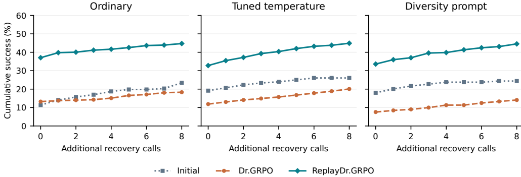
Figure 25: Recovery after independently chosen feasible Pantry outages. Zero additional calls measures survival of the eight saved plans. Subsequent points include successful recovery within the displayed call budget. Trained curves average fixed seeds 43 and 46; initial-model curves use one checkpoint. All panels use the same 32 problems; paired uncertainty appears in Table 60.
