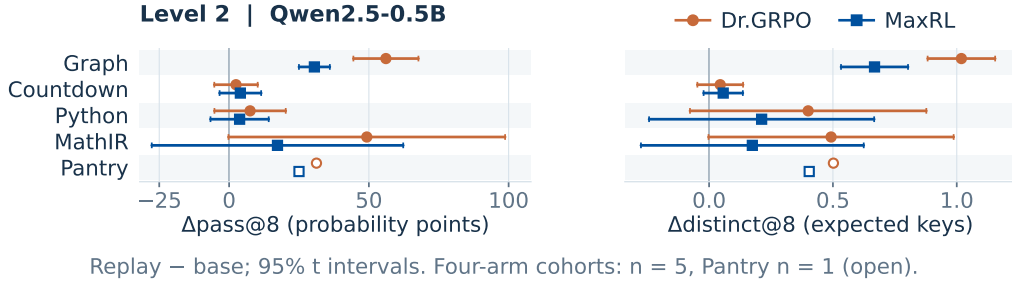
Figure 12: Replay effects within Level 2. Replay and control are compared on the same prompts and training seeds, with separate Dr.GRPO and MaxRL effects. Four domains have complete factorials; PantryPlan retains its partial counts and descriptive effects. Construction and admission are described in Section 2.2; terminal absolute values appear in Figure 7. Differences between levels combine task, population, and protocol changes, so they do not identify a causal effect of difficulty alone.
