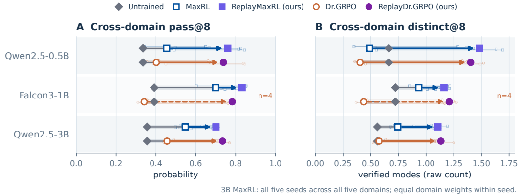
Figure 5: MaxRL and replay at all three model scales. Tracks connect initial, trained, and replay models. Complete tracks average within seed. All MaxRL tracks use five paired seeds in every domain, including 3B; Falcon Dr.GRPO uses four common seeds. Archived models.
