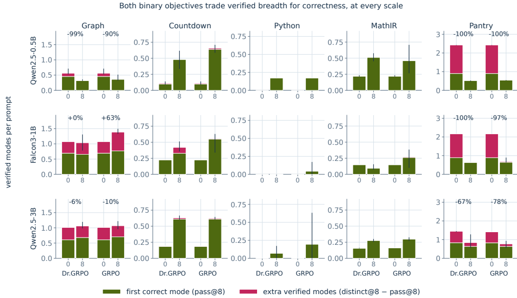
Figure 15: Verifier-only training reduces average extra verified modes at each tested scale. Bars split \text{distinct@8} into the first correct mode and every verified mode beyond it, at training pass 0 and pass 8, for unmodified Dr.GRPO then GRPO in each panel. All 150 evaluations are complete at five seeds and four fixed K = 8 draws; whiskers are the seed range and pass 0 is measured per method. Badges give the change in extra verified modes, printed only where pass-0 breadth exceeds .05 of them; the other three domains start at .011 or less.
