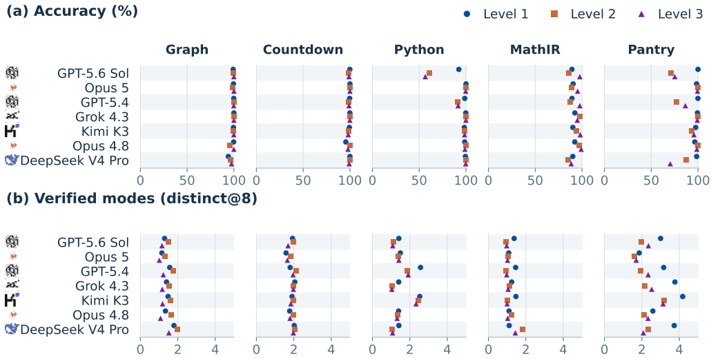
Figure 23: Accurate hosted outputs can still cover few verified modes. Columns show domains; markers distinguish Levels 1–3. Each point uses all eight responses to each of 128 prompts. Top: per-response accuracy. Bottom: distinct@8. A fixed formatting normalizer applies to every deployment; Opus 5 Python uses revised task wording without a system message. Table 1 reports per-level averages of pass@8 and distinct@8 across all five domains.
