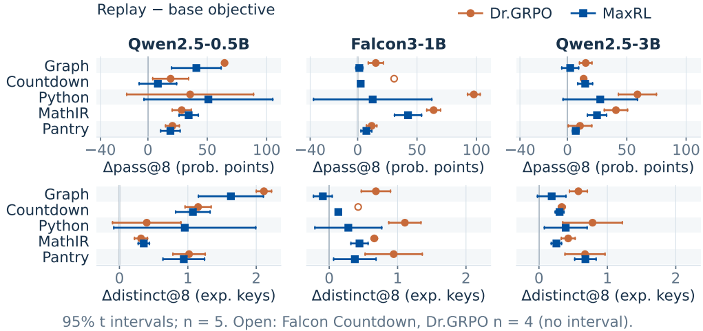
Figure 9: Canonical replay complements both fresh objectives. Each point compares replay with its matched no-replay control at pass eight, within domain and scale. The two endpoints have different units: success probability points and expected verified-key counts. All 75 MaxRL pairs are complete; Falcon Countdown uses four Dr.GRPO pairs and all other Dr.GRPO blocks use five. Nominal intervals accompany complete blocks only. Domain variation is retained; these comparisons identify the implemented replay addition rather than a universal benefit or factorial interaction.
