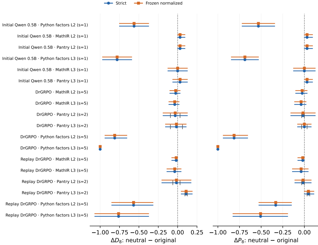
Figure 25: Prompt-hint removal effects for local checkpoints, preserving every registered domain-level cell. Blue circles use strict verification; orange squares use the same frozen formatting normalizer. Horizontal bars show the intervals described in the tables; zero is the vertical reference. Gray end-point marks show the two individual Pantry seed effects.
