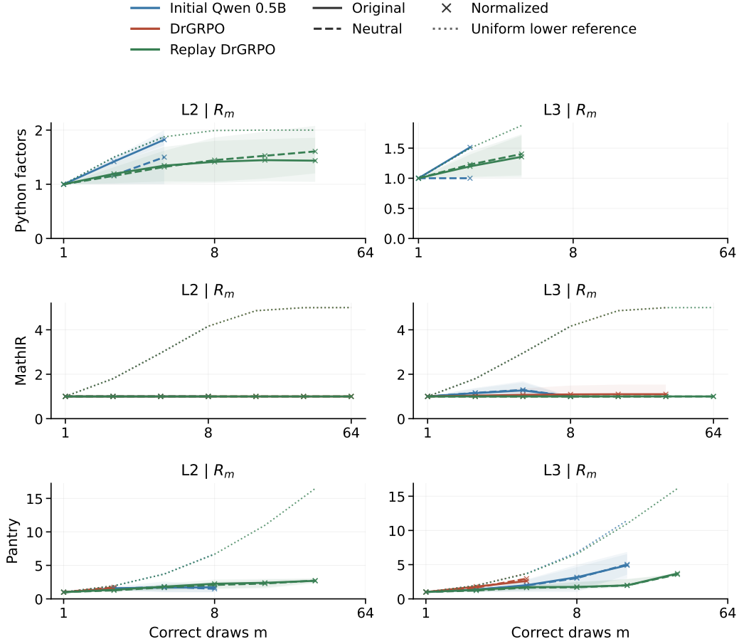
Figure 27: Breadth after exactly m correct draws, on prompts jointly eligible under both wordings. Color and solid/dashed wording styles match the discovery figure; dotted lines give method-specific uniform lower references using the same eligible prompts. Undefined means are gaps. Crosses show frozen normalization. Eligibility varies with m , so curves do not hold the eligible population fixed across the horizontal axis; the following table gives all strict joint counts for every method, level, and correct-draw budget, including groups with zero eligible prompts.
