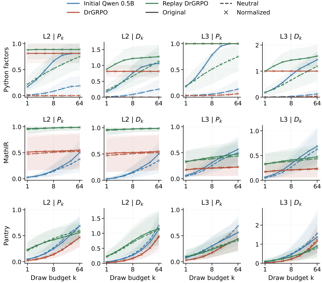
Figure 26: Fresh 64-draw discovery curves. Separate axes show P_k and D_k for each level and domain; pass probability always uses a 0–1 scale. Color identifies the checkpoint method or hosted model, solid/dashed lines original/neutral wording. Lines and shaded pointwise intervals use strict grading; crosses show the frozen-normalization sensitivity. Prefix estimates are separately retained in the report with pointwise intervals for every model and cell.
