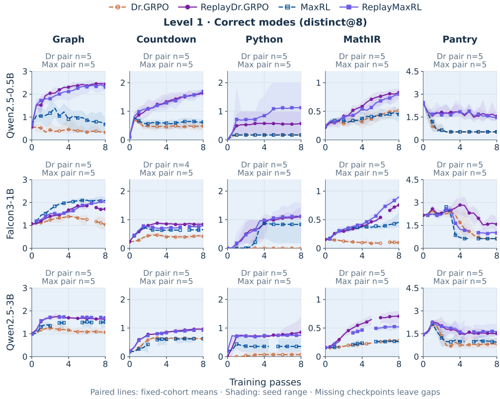
Figure 13: Verified modes throughout training at all three model scales. The same model rows, methods, seeds, and checkpoints as Figure 12, now measuring distinct@8 . Lines are descriptive fixed-cohort means and bands show seed ranges. A count of one has no band. Domain-specific vertical scales are shared across model rows; absolute heights across different domains should be read against their labeled axes. Missing evaluations are never carried forward or joined across a gap.
