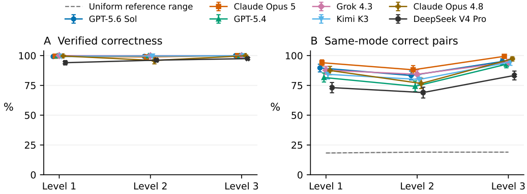
Figure 22: Verified correctness and concentration in hosted Graph outputs. Each deployment receives the same 128 prompts per level, with eight stateless samples per prompt. Intervals resample whole prompts. The gray band spans the models’ uniform-correct-key references, conditional on their observed correct draws. Graph was selected after the GPT-5.6 Sol run and before the prospective comparison runs. Level labels do not guarantee increasing difficulty for each model.
