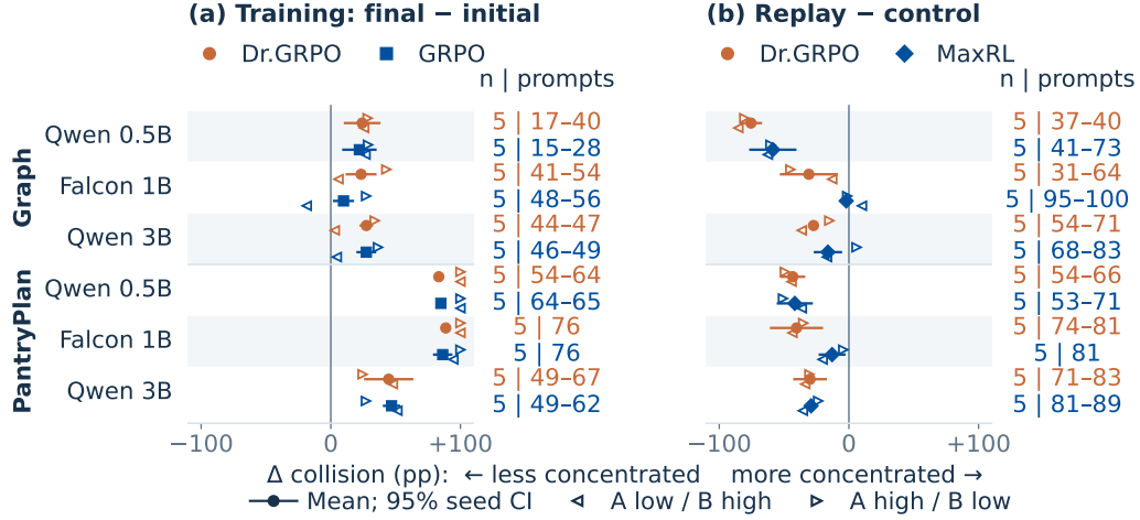
Figure 19: Training concentrates verified outputs; canonical replay can mitigate it. Left: final minus initial correct-key collision for Dr.GRPO and GRPO. Right: replay minus its matched terminal control, separately for Dr.GRPO and MaxRL. Graph and PantryPlan have substantial initial breadth. Dots and nominal 95% intervals average five seed contrasts; each contrast weights jointly eligible prompts equally. Smaller markers show the two disjoint-stream orientations; gutters give defined seed n and the eligible-prompt count range out of 128. The two panels have separate eligibility and are not one trajectory. Appendix H.1 reports all five domains, undefined cells, source assumptions, and correctness changes on the same eligible prompts.
