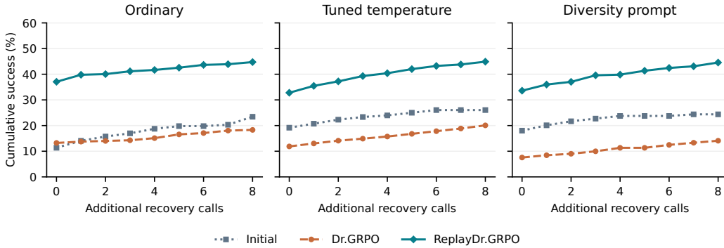
Figure 24: Recovery after independently chosen feasible Pantry outages. Zero additional calls measures survival of the eight saved plans. Subsequent points include successful recovery within the displayed call budget. Trained curves average fixed seeds 43 and 46; initial-model curves use one checkpoint. All panels use the same 32 problems; paired uncertainty appears in Table 57.
