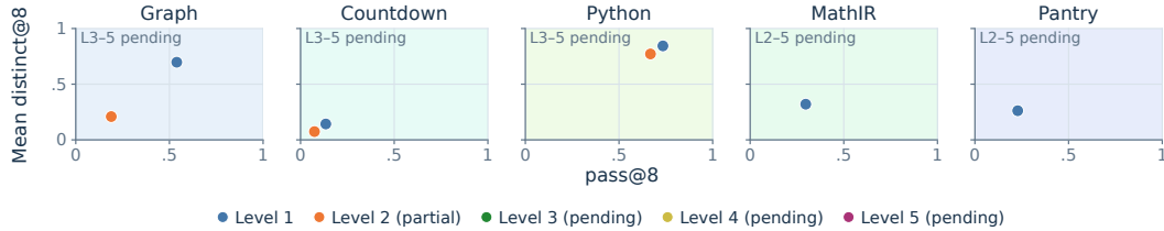
Figure 3: Frozen-model success and breadth across levels. Five domains, with pass@8 versus mean distinct verified modes per eight draws; colors identify levels for Qwen2.5-0.5B-Instruct. Each point averages four independent eight-draw groups on 128 held-out prompts at T = 1 . Eight of 25 cells are measured. Level-2 MathIR/Pantry and Level 3 await evaluation; Levels 4–5 await dataset admission. Only completed measurements are plotted.
