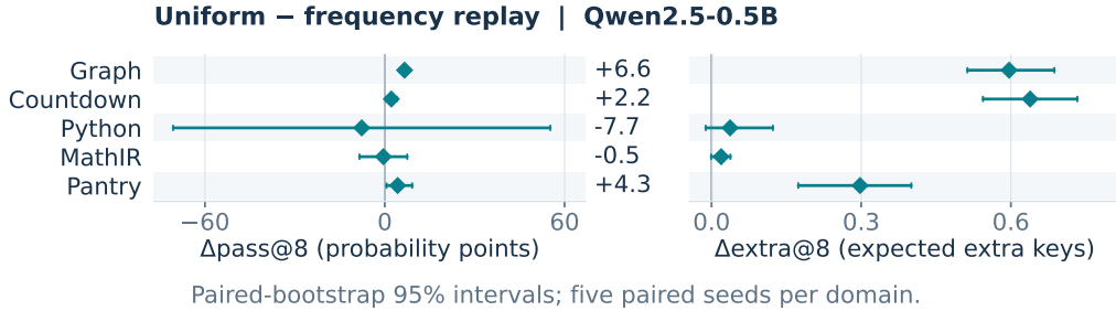
Figure 18: Equal key weights can improve breadth beyond the first success. Uniform minus fresh-frequency weighting of verified replay. Success and extra modes are separate endpoints; a positive extra-mode effect does not hold correctness fixed. The displayed model, domains, seeds, and uncertainty use the frozen weighting comparison. The domain variation and inconclusive success contrast limit the claim to the demonstrated breadth contribution.
