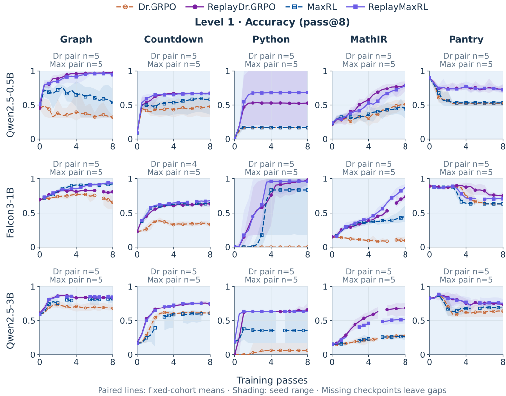
Figure 12: Accuracy throughout training at all three model scales. Rows are Qwen2.5-0.5B, Falcon3-1B, and Qwen2.5-3B; columns are the five domains. Dr.GRPO, ReplayDr.GRPO, MaxRL, and ReplayMaxRL use the same method colors as Figure 6. Lines are fixed-cohort means of pass@8 ; bands are seed ranges, not confidence intervals. Counts identify each objective’s terminal paired seeds. Qwen2.5-3B MaxRL uses all five seeds in every domain; Falcon Countdown Dr.GRPO/replay uses four. Gaps indicate missing or conflicting checkpoints.
