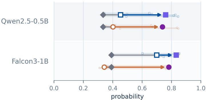
A Cross-domain pass@8
