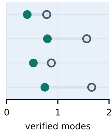
distinct@8
