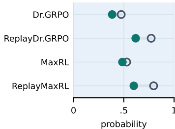
pass@8
