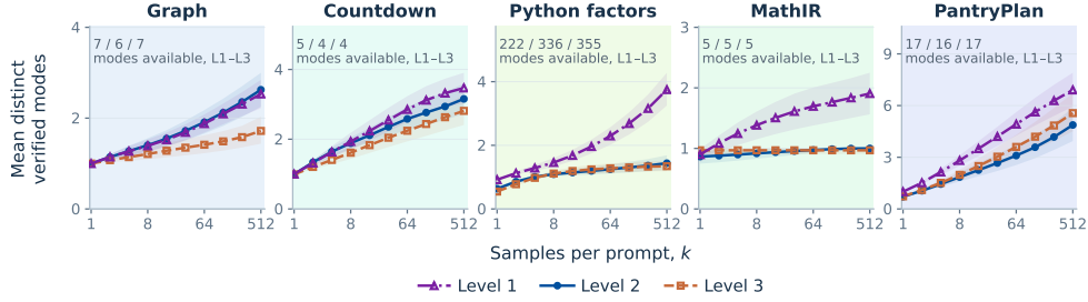
Figure 4: More samples need not recover the available modes. GPT-5.6 Sol, medium reasoning; 32 problems per domain and level, 512 responses each. Curves average distinct verified modes in random k -subsets, including failures; bands are pointwise 95% problem-bootstrap intervals. The figure prints how many modes each panel’s problems actually admit, averaged over the problems used, in Level 1 / Level 2 / Level 3 order; the counts are the enumerated support the benchmark registers with each problem, so the gap between a curve and its count is what the model never produced (App. K.3).
