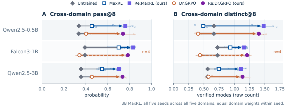
Figure 7: Replay complements both fresh objectives at multiple scales. Each row shows Dr.GRPO/Re:Dr.GRPO and MaxRL/Re:MaxRL on both endpoints. Diamonds are initial models; open/filled markers are training without/with replay. Tracks average domains within seed; faint paths show seeds. All MaxRL tracks use five paired seeds in all five domains, including 3B. Falcon Dr.GRPO uses four common seeds; the other Dr.GRPO tracks use five. App. Fig. 13 reports each domain’s correctness and verified-mode results at every scale.
