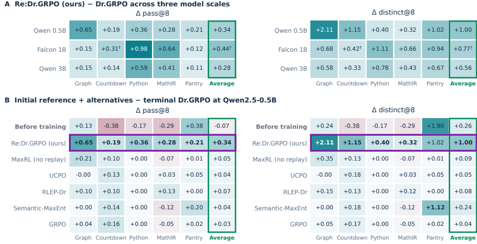
Figure 6: Canonical replay improves correctness and verified breadth. (A) Re:Dr.GRPO minus Dr.GRPO at all three scales. (B) Qwen2.5-0.5B alternatives minus Dr.GRPO. Columns measure probability points and expected verified-mode counts, respectively. The green Average weights domains equally within seed. A dagger marks four paired seeds in Falcon Countdown and its Average; other cells use five. Intervals are nominal 95% intervals for five-seed comparisons. Purple denotes Re:Dr.GRPO; bold entries mark column maxima in Panel B.
