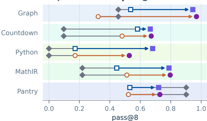
A Qwen2.5-0.5B · pass@8
