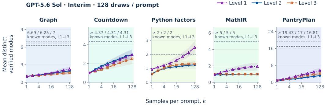
Figure 8: More samples need not recover the available modes. GPT-5.6 Sol; all five domains and Levels 1–3, with sixteen problems per cell. Interim 128-response pools; the 512-draw run continues. Curves show mean distinct verified modes in random k -subsets; bands are pointwise 95% problem-bootstrap intervals. Gray lines show mean known support: exact for Graph, certified lower bounds elsewhere. Formatting normalization and collection details appear in Appendix N.4.
