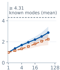
Countdown
