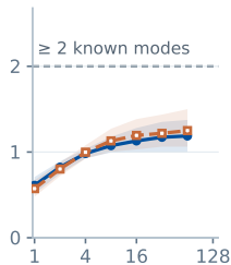
Python factors
