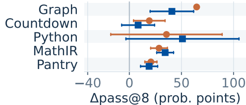
Qwen2.5-0.5B
