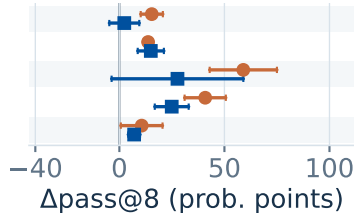
Qwen2.5-3B
