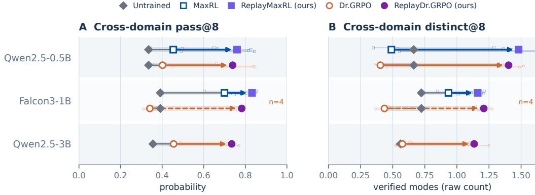
Figure 5: Memory adds value beyond sampling-aware MaxRL. Each track connects the untrained model, fresh-objective training, and its replay counterpart. Faint paths are seeds; bold paths average four domains within seed. Falcon Dr.GRPO uses four common admissible seeds; other tracks use five. The Qwen2.5-3B row shows its completed Dr.GRPO/replay track.
