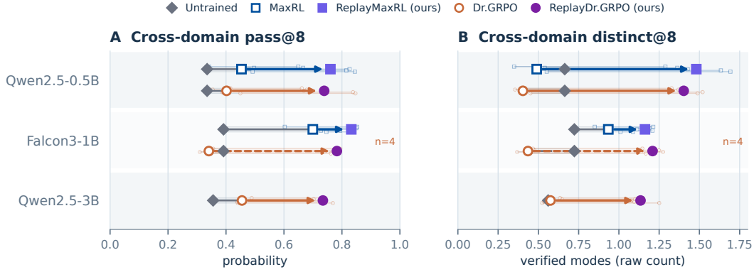
Figure 5: Memory adds value beyond sampling-aware MaxRL. Each track connects the untrained model, fresh-objective training, and its replay counterpart. Faint paths are seeds; bold paths average domains within seed. Falcon Dr.GRPO uses four common admissible seeds; other tracks use five. The Qwen2.5-3B row shows its completed Dr.GRPO/replay track.
