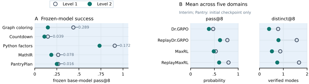
Figure 6: Replay across difficulty levels with Qwen2.5-0.5B-Instruct. Open/filled markers: Level 1/2. (A) Frozen-model success. (B) Interim means weight the five domains equally after averaging seeds. Checkpoints match across levels and methods; Pantry has one seed at step 0 (Appendix N.1).
