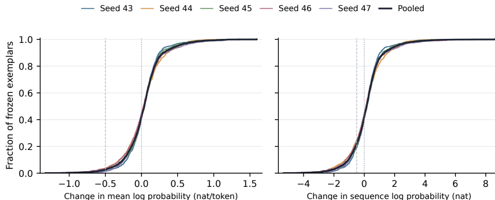
Figure 13: Fixed-exemplar scores improve centrally but retain a declining tail. Empirical cumulative distributions show first-to-final post-freeze score changes for every frozen identity, with one curve per seed and the pooled identity distribution. Mean token and sequence scores are separate panels; positive values indicate increased teacher-forced likelihood. Neither panel measures the exact probability of generating a canonical mode during policy sampling.
