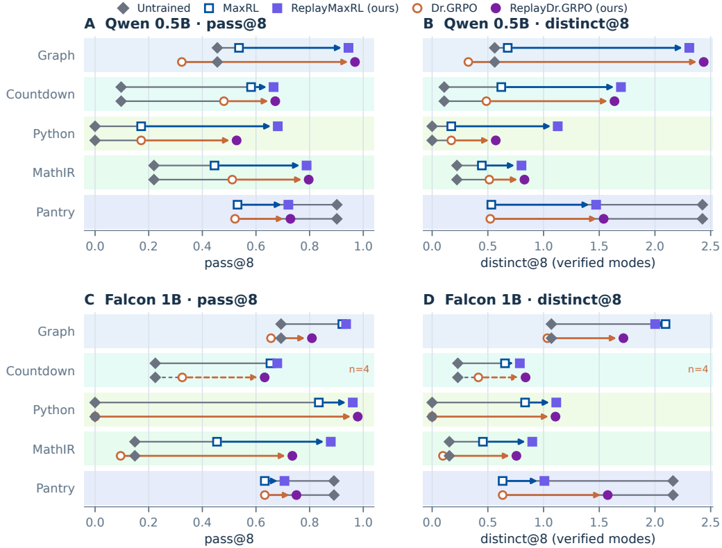
Figure 14: Per-domain results behind the cross-domain averages in Figure 5. Panels A–B show Qwen2.5-0.5B and panels C–D show Falcon3-1B. MaxRL–ReplayMaxRL pairs retain five terminal seeds in every domain. Dr.GRPO–ReplayDr.GRPO uses four admissible seeds for Falcon Countdown and five elsewhere. Domain tints match Figure 2. Replay arrows, trained-arm markers, and untrained references use the same encoding as the main figure.
