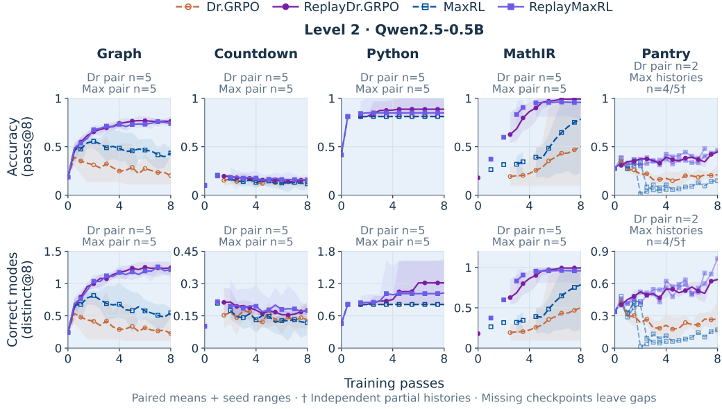
Figure 9: Accuracy and verified modes during Level-2 training. Qwen2.5-0.5B is the model tested at this level. Rows show pass@8 and distinct@8 for all four primary methods. Graph, Countdown, Python, and MathIR contain five terminal paired seeds per objective. PantryPlan’s Dr.GRPO/replay means use their two terminal paired seeds; additional MaxRL and ReplayMaxRL histories are individual, unpaired observations, marked separately without a mean or band. They do not estimate a paired replay effect. Both metrics follow the same evaluation rules, with gaps at missing checkpoints and no extrapolation to later training passes.
