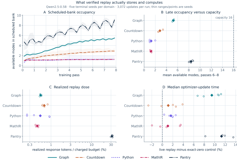
Figure 16: The verified replay path is active and bounded. Telemetry summarizes all 25 terminal Qwen2.5-0.5B ReplayDr.GRPO runs and their matched controls. It records bank availability and occupancy, capacity hits, realized replay-token dose, and paired optimizer time. These measurements validate the intervention but do not by themselves establish causal mediation through any individual stored mode across training checkpoints.
