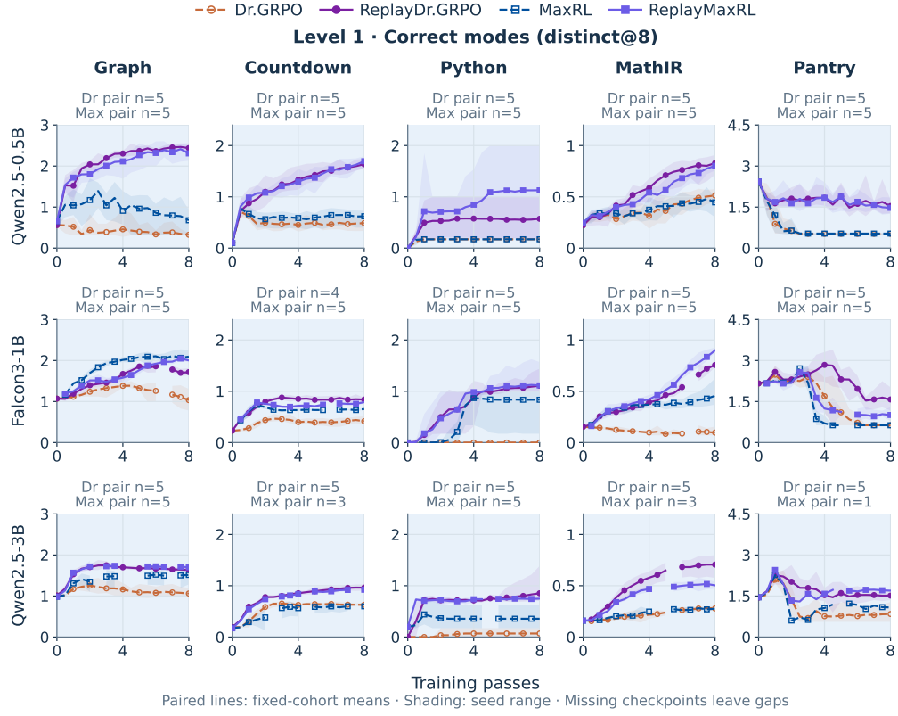
Figure 8: Verified modes throughout training at all three model scales. The same model rows, methods, seeds, and checkpoints as Figure 7, now measuring distinct@8. Lines are descriptive fixed-cohort means and bands show seed ranges. A count of one has no band. Domain-specific vertical scales are shared across model rows; absolute heights across different domains should be read against their labeled axes. Missing evaluations are never carried forward or joined across a gap.
