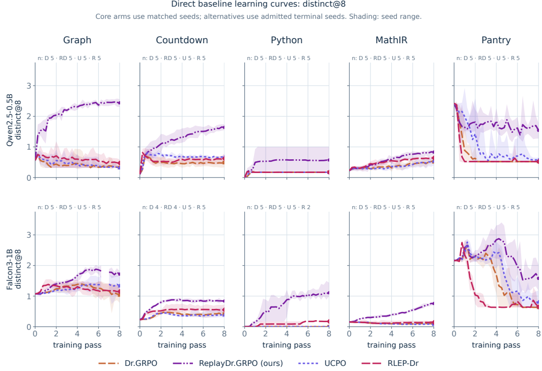
Figure 12: Verified-mode trajectories for the supporting comparators. Rows show Qwen2.5-0.5B and Falcon3-1B; columns are the five domains. UCPO and sparse RLEP-Dr are compared with Dr.GRPO and ReplayDr.GRPO at these two smaller scales. Labels give exact method-specific seed counts. Lines are descriptive distinct@8 means and bands are seed ranges. The corresponding accuracy curves use identical populations in Figure 13.
