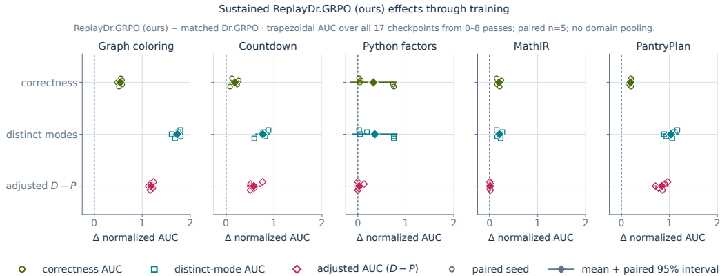
Figure 10: Sustained ReplayDr.GRPO effects through training. Qwen2.5-0.5B ReplayDr.GRPO is compared with matched Dr.GRPO separately on each static domain. Effects are trapezoidal trajectory AUCs over all 17 registered half-pass checkpoints from 0 through 8 passes, divided by the eight-pass horizon. Open markers are the five paired seeds 43–47, diamonds are paired means, and bars are unadjusted descriptive two-sided 95% Student- t estimation intervals. The adjusted effect subtracts correctness AUC from distinct-mode AUC per seed. No significance decision is made for an individual model–domain comparison, and no checkpoint, domain, or metric magnitude is pooled. An early-collapsed control can remain flat for most of the horizon, so AUC partly measures time spent in that state and is a sensitivity analysis, not independent mechanism evidence.
