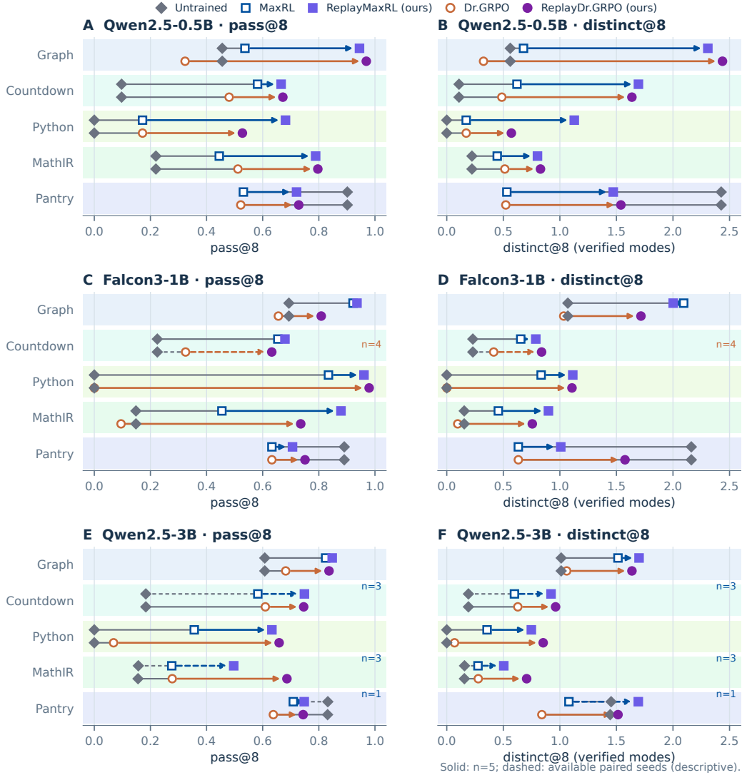
Figure 18: Per-domain results behind the cross-domain averages in Figure 5. Rows show Qwen2.5-0.5B, Falcon3-1B, and Qwen2.5-3B; columns show correctness and raw support. MaxRL–ReplayMaxRL pairs retain five terminal seeds throughout the two smaller models. Qwen2.5-3B uses n = 5, 3, 5, 3, 1 in domain order; dashed connectors mark partial blocks. Dr.GRPO–ReplayDr.GRPO uses four admissible seeds for Falcon Countdown and five elsewhere. Domain tints match Figure 2. Replay arrows, trained-arm markers, and untrained references use the same encoding as the main figure.
