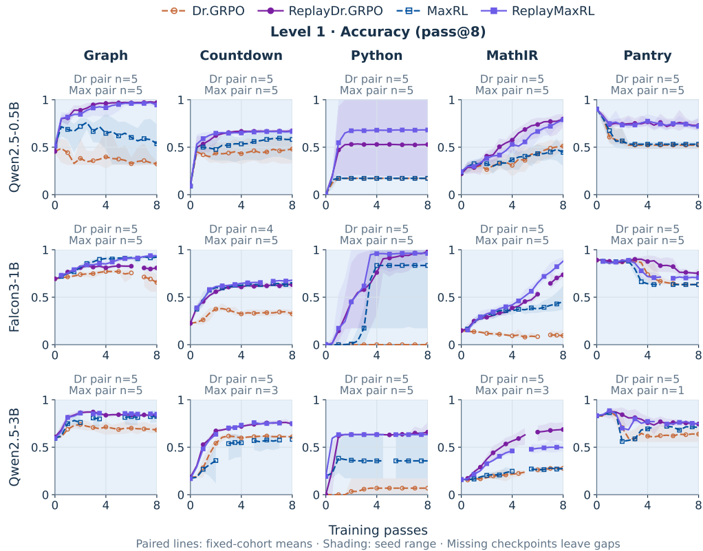
Figure 7: Accuracy throughout training at all three model scales. Rows are Qwen2.5-0.5B, Falcon3-1B, and Qwen2.5-3B; columns are the five domains. Dr.GRPO, ReplayDr.GRPO, MaxRL, and ReplayMaxRL use the same method colors as Figure 5. Lines are fixed-cohort means of pass@8; bands are seed ranges, not confidence intervals. Counts identify each objective’s terminal paired seeds. Qwen2.5-3B MaxRL retains Graph/Countdown/Python/MathIR/Pantry counts 5/3/5/3/1; Falcon Countdown Dr.GRPO/replay uses four. Gaps indicate missing or conflicting checkpoints.
