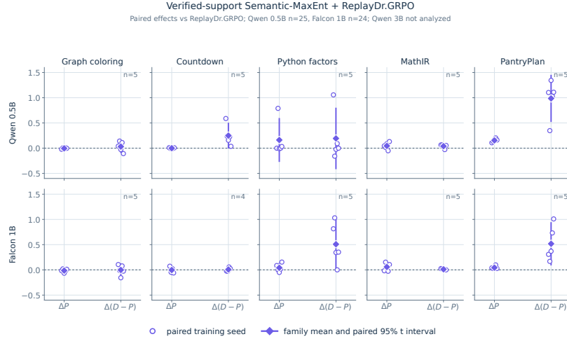
Figure 15: Bundled verified-support comparison. Effects compare ReplayDr.GRPO augmented with semantic regularization and proposal sampling against ReplayDr.GRPO after eight passes. Qwen uses n = 5 ; Falcon uses n = 5 except Countdown ( n = 4 ). The historical exploratory amendment retains its n = 4 interval policy, separately from the primary analyses (Appendix F.1). This bundled historical comparison is supporting evidence, not a component of the primary ReplayMaxRL intervention evaluated here.
