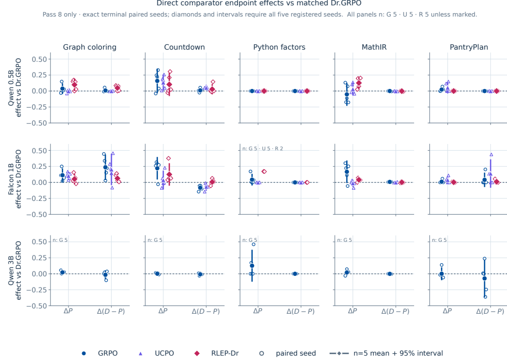
Figure 23: Direct alternatives produce local rather than uniform final gains. Each effect subtracts the same-seed Dr.GRPO control from the comparator after eight passes. Effects are shown for \text{pass}@8 and extra verified modes beyond the first success. Circles are paired seeds; diamonds and 95% Student- t intervals appear only for complete five-seed blocks. Exact n is printed, and unsupported comparisons remain blank rather than being extrapolated or imputed at any seed.
