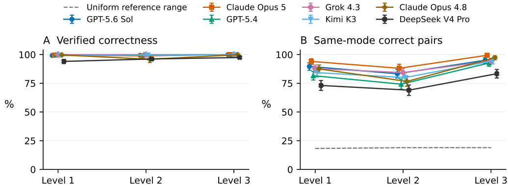
Figure 35: Verified correctness and concentration in hosted Graph outputs. Each deployment receives the same 128 prompts per level, with eight stateless samples per prompt. Intervals resample whole prompts. The gray band spans the models’ uniform-correct-key references, conditional on their observed correct draws. Graph was selected after the GPT-5.6 Sol run and before the prospective comparison runs. Level labels do not guarantee increasing difficulty for each model.
