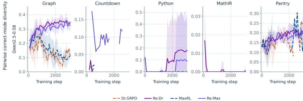
Figure 22: Verified-mode diversity during Level-2 training. The same model, methods, seeds, and checkpoints as Fig. 21, measuring PCMD. Graph separates the arms most clearly: both replay arms rise to roughly .34 while Dr.GRPO and MaxRL fall to near .11, so the replayed policies end with about three times the chance that two verified colorings differ. MathIR collapses to PCMD .000 under every arm at this level. Level-2 support is thin in Countdown and Python, where only the steps clearing 30 defined prompts are drawn and segments are not joined across the rest.
