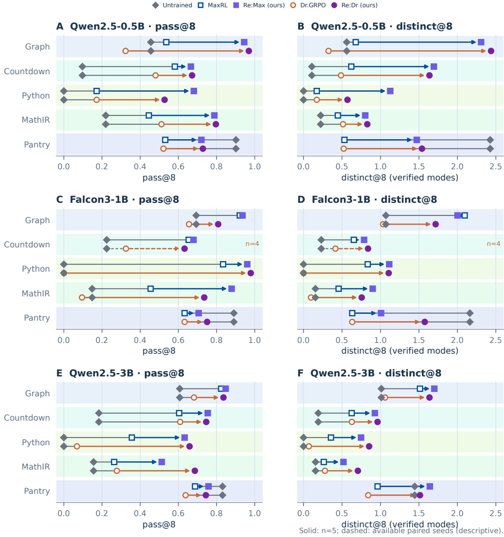
Figure 16: Per-domain results behind the cross-domain averages in Fig. 8. Rows show Qwen2.5-0.5B, Falcon3-1B, and Qwen2.5-3B; columns show correctness and raw support. MaxRL–Re:Max pairs retain five terminal seeds throughout the two smaller models and Qwen2.5-3B: every MaxRL domain uses n = 5 . Solid connectors identify these complete comparisons. Dr.GRPO–Re:Dr uses four admissible seeds for Falcon Countdown and five elsewhere. Domain tints match Fig. 2. Replay arrows, trained-arm markers, and untrained references use the same encoding as Fig. 8. The E118 model index groups the archived exports by model and domain.
