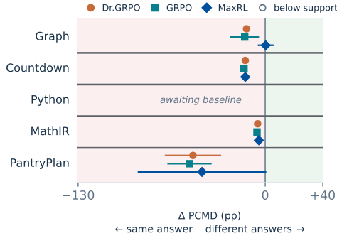
Figure 7: Training concentrates verified outputs. Final minus initial PCMD at Qwen2.5-3B under three objectives, five domains, from the independently seeded resampling: both sides of the difference are measured on the same surface. Marks are means over training seeds with nominal 95% intervals. Eleven of the twelve measurable comparisons move left; the exception is within half a point of zero. Other scales and every level: Fig. 14; counts: App. G.1.
