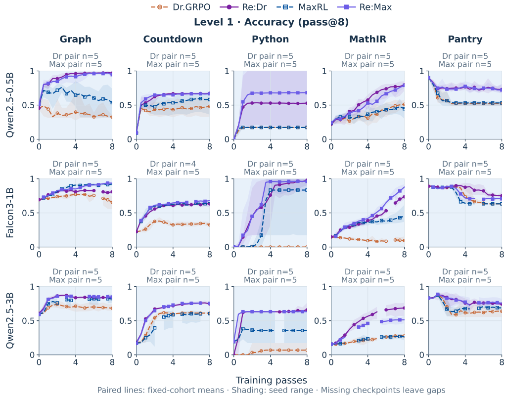
Figure 18: Accuracy throughout training at all three model scales. Rows are Qwen2.5-0.5B, Falcon3-1B, and Qwen2.5-3B; columns are the five domains. Dr.GRPO, Re:Dr, MaxRL, and Re:Max use the same method colors as Fig. 8. Lines are fixed-cohort means of pass@8; bands are seed ranges, not confidence intervals. Counts identify each objective’s terminal paired seeds. Qwen2.5-3B MaxRL uses all five seeds in every domain; Falcon Countdown Dr.GRPO/replay uses four. Gaps indicate checkpoints that are missing or whose provenance conflicts, and are left unjoined rather than interpolated across, so a break in a line is an absence of admissible evidence at that step rather than a measured value of zero for that arm at that checkpoint.
