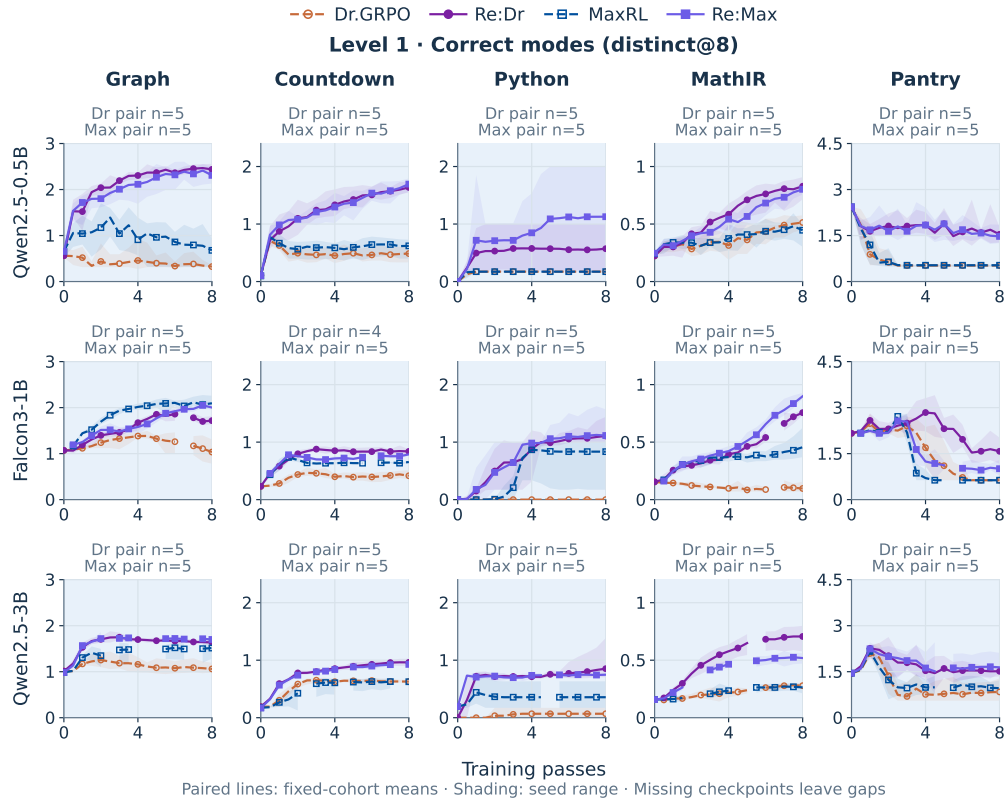
Figure 20: Registered verified-mode counts throughout training. The same rows, methods, seeds, and checkpoints as Fig. 19, measuring the registered distinct@8 rather than PCMD. It is retained because distinct@8 is a registered co-primary endpoint. Read against the panel above, it also shows why the success-conditional axis is reported alongside it: curves that rise here can do so because correctness rose, and the two figures separate in exactly the cells where they do. Lines are descriptive fixed-cohort means and bands show seed ranges. A count of one has no band. Missing evaluations are never carried forward or joined across a gap.
