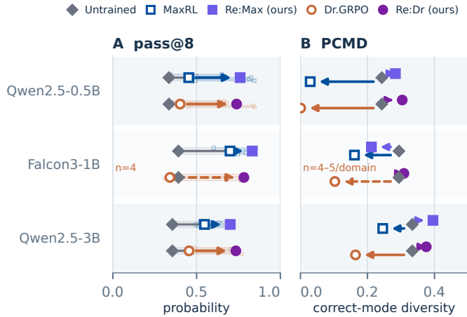
Figure 8: Replay complements both fresh objectives at multiple scales. Diamonds are initial models; open/filled markers are training without/with replay. (A) averages all five domains within seed; faint paths show seeds. (B) draws both arrows from the untrained model — one to the fresh objective alone, one to it with memory — over the domains where every arm clears the support bar. Solid arrows are complete five-seed blocks; thinner pairs print their counts. App. Fig. 16 gives each domain at every scale.
