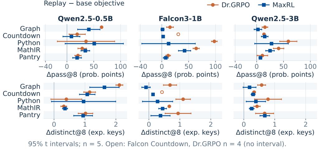
Figure 15: Canonical replay complements both fresh objectives. Each point compares replay with its matched no-replay control at pass eight, within domain and scale. The two endpoints have different units: success probability points and expected verified-key counts. All 75 MaxRL pairs are complete; Falcon Countdown uses four Dr.GRPO pairs and all other Dr.GRPO blocks use five. Nominal intervals accompany complete blocks only. Domain variation is retained; these comparisons identify the implemented replay addition rather than a universal benefit or factorial interaction.
