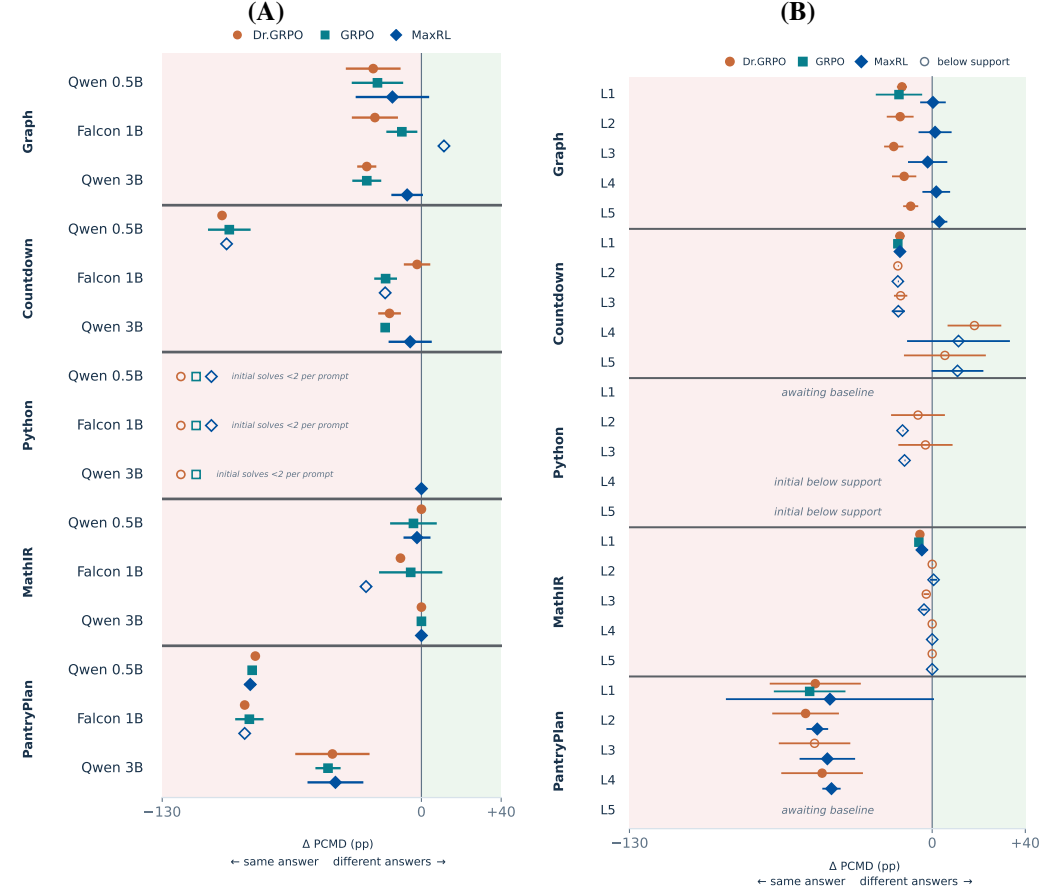
Figure 14: Concentration along both axes. (A) Concentration at every scale. Fig. 7 for all three scales rather than Qwen2.5-3B alone: final minus initial PCMD under Dr.GRPO, GRPO and MaxRL, five domains by three scales. Marks are means over five seeds with nominal 95% seed intervals; open marks carry fewer than five seeds and no interval, or name an objective PCMD cannot score because the initial checkpoint returns two correct responses to no prompt. The scale ordering is the same one Fig. 3 uses. (B) Training narrows breadth on constructions it never trained on. Final minus initial PCMD for Qwen2.5-3B policies trained at Level 1 and read on each level’s held-out split, so every row above L1 is transfer rather than training at that level. Marks are means over training seeds against the one untrained checkpoint per cell, with nominal 95% seed intervals; the spread is across seeds, not a paired design. Open marks fall below the support bar, where the estimate stands but its precision does not. Dr.GRPO narrows at every level while MaxRL stays near zero, and Countdown crosses to the broadening side by Levels 4 and 5 — the direction is not a property of training alone but of training and construction together. Rows marked awaiting a baseline have no untrained measurement on that split yet.
