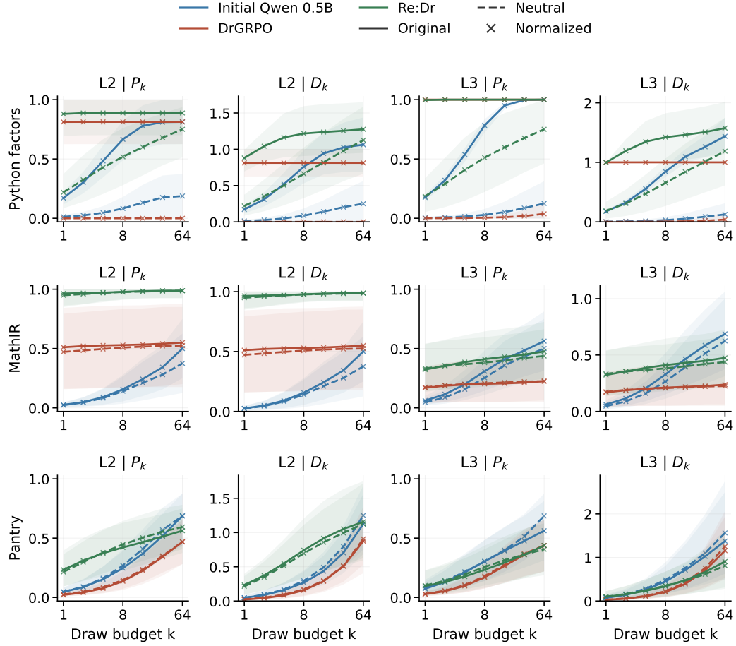
Figure 32: Fresh 64-draw discovery curves. Separate axes show P_k and D_k for each level and domain; pass probability always uses a 0–1 scale. Color identifies the checkpoint method or hosted model, solid/dashed lines original/neutral wording. Lines and shaded pointwise intervals use strict grading; crosses show the frozen-normalization sensitivity. Prefix estimates are separately retained in the report with pointwise intervals for every model and cell.
