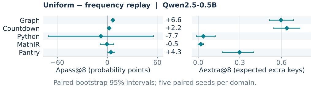
Figure 26: Equal key weights can improve breadth beyond the first success. Uniform minus fresh-frequency weighting of verified replay. Success and extra modes are separate endpoints; a positive extra-mode effect does not hold correctness fixed. The displayed model, domains, seeds, and uncertainty use the frozen weighting comparison. The domain variation and inconclusive success contrast limit the claim to the demonstrated breadth contribution.
