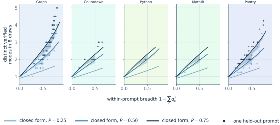
Figure 10: The decomposition against measured prompts, by domain. Bands are the closed form above, \sum_c [1 - (1 - Pq_c)^8] , evaluated over allocations from a point mass to uniform; at each breadth a band spans only the key counts that can attain it, over the range those prompts realize. Points are 1,092 held-out prompts returning at least two verified responses, at the terminal checkpoint of the Qwen2.5-0.5B replay arms, binned by measured verified mass P . Panels are the five domains and carry the tints of their cards in Fig. 2, because a mode means something different in each and the number of keys a prompt can occupy is a property of the domain. Graph and Pantry occupy the full range; Python and MathIR sit at the left edge, MathIR almost entirely so — nearly every one of its prompts returns a single key, where two correct answers are the same answer. Occupied keys stay far below the bank capacity of M = 16 : what bounds these policies is how many modes they find, not how many the bank can hold.
