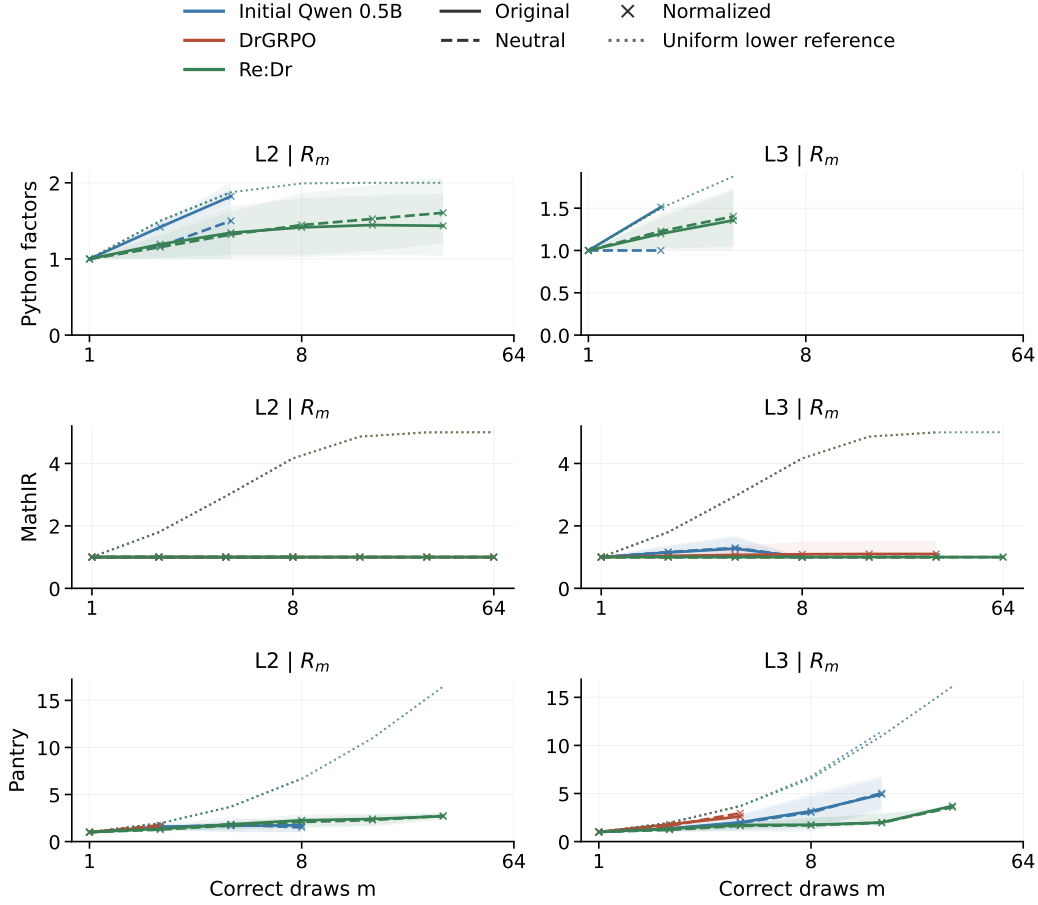
Figure 33: Breadth after exactly m correct draws, on prompts jointly eligible under both wordings. Color and solid/dashed wording styles match the discovery figure; dotted lines give method-specific uniform lower references using the same eligible prompts. Undefined means are gaps. Crosses show frozen normalization. Eligibility varies with m , so curves do not hold the eligible population fixed across the horizontal axis; the following table gives all strict joint counts for every method, level, and correct-draw budget, including groups with zero eligible prompts.
