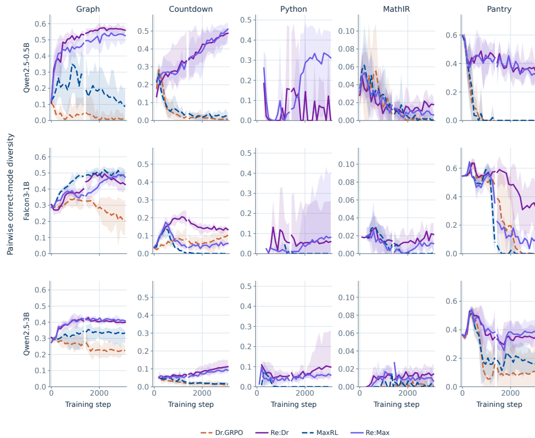
Figure 19: Verified-mode diversity throughout training at all three model scales. The same model rows, methods, seeds, and checkpoints as Fig. 18, now measuring PCMD. Because the metric conditions on the verified draws, a falling line reports that successes concentrated, not that they became rarer — the distinction the accuracy curves cannot draw. The two fresh objectives fall in Graph, Countdown, and Pantry at every scale, reaching PCMD .000 in Pantry at 0.5B and 1B, while the replay arms rise or hold. Lines are descriptive fixed-cohort means and bands show seed ranges. A count of one has no band. Domain-specific vertical scales are shared across model rows; absolute heights across different domains should be read against their labeled axes. A step is plotted only where at least 30 prompts return two verified responses, and segments are never joined across a suppressed step, so a gap in a line marks a step whose breadth could not be measured on enough prompts rather than a step at which breadth was measured and found to be zero.
