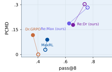
Figure 9: Replay across difficulty levels at Qwen2.5-0.5B. Open/filled markers denote Level 1/2; both levels and all four methods share five paired seeds. \text{pass@8} averages all five domains; PCMD averages the two — Graph and MathIR — where every method clears the support bar at both levels, so no arm rests on an easier subset (App. E.3).
