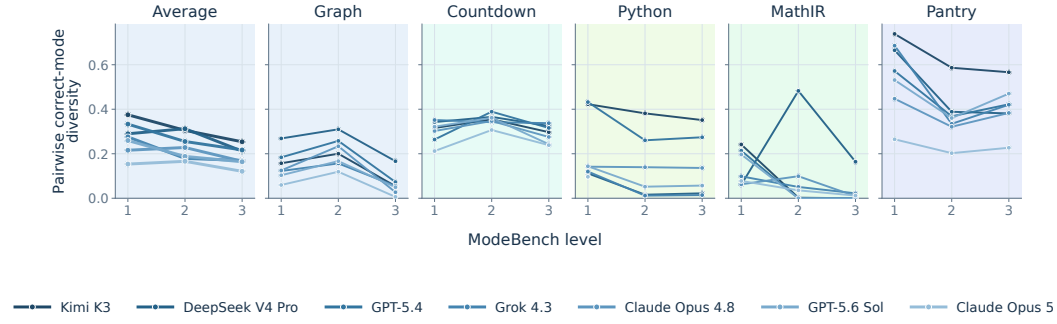
Figure 12: Harder levels narrow the frontier. Success-conditional breadth against the ladder, one line per hosted deployment, over 128 held-out prompts and eight stateless requests per prompt per cell. Colour runs with collapse, darkest most concentrated. Only the rungs every deployment covers are drawn: Levels 4 and 5 exist for one deployment alone, and a line running past its neighbours would read as that deployment holding up where the others fall rather than as the only one measured there (App. L.1 reports those two probes separately). Correctness is not drawn, because there is nothing to see — every hosted cell sits above pass@8 .898, so the ladder costs these deployments accuracy they do not have to give and breadth they do. The Average panel weights domains equally over a set held fixed for each deployment, so the domain mix cannot move with the level; on it every one of the seven falls from Level 1 to Level 3, by .033 to .121. The domains do not agree on how: MathIR runs to zero, Python and Graph fall, and Countdown does not narrow at all. Open marks sit below the support bar and stay off the line.
