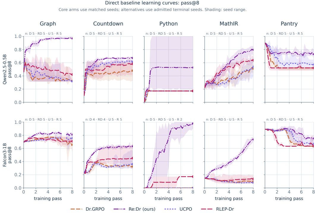
Figure 25: Accuracy trajectories for the supporting comparators. The same model rows, domains, methods, terminal seeds, and registered checkpoints as Fig. 24, now measuring pass@8. Bands show the seed range and the vertical axes span [0, 1] throughout. MaxRL and Re:Max at all three scales are compared on both metrics in Figs. 18 and 19.
