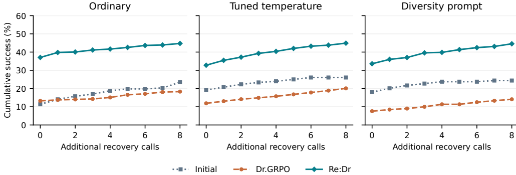
Figure 34: Recovery after independently chosen feasible Pantry outages. Zero additional calls measures survival of the eight saved plans. Subsequent points include successful recovery within the displayed call budget. Trained curves average fixed seeds 43 and 46; initial-model curves use one checkpoint. All panels use the same 32 problems; paired uncertainty appears in Table 43.
