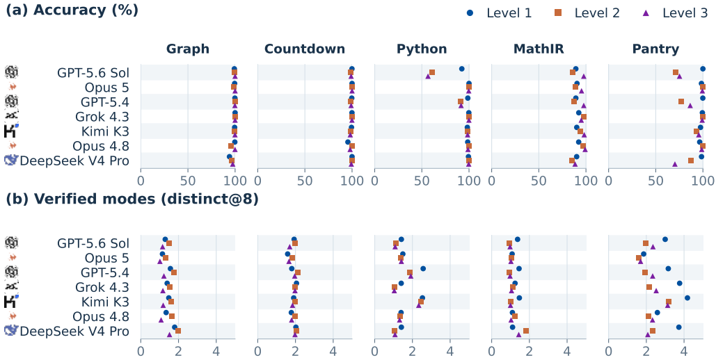
Figure 37: Accurate hosted outputs can still cover few verified modes. Columns show domains; markers distinguish Levels 1–3. Each point uses all eight responses to each of 128 prompts. Top: per-response accuracy. Bottom: distinct@8. A fixed formatting normalizer applies to every deployment; Opus 5 Python uses revised task wording without a system message. Table 81 reports the corresponding per-level averages of pass@8 and distinct@8 across all five domains.
