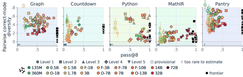
Figure 13: Four model families on the axes of Fig. 3. Frozen instruction-tuned models from SmoLM2, Qwen2.5, Falcon3 and OLMo-2, plotted as pass@8 against PCMD; colour runs green to red with parameter count on a log scale, and marker shape identifies the level. This figure carries every model family and every level collected, where Fig. 3 shows Qwen2.5 alone. Grey markers are all 7 hosted deployments of Section 2.3, of which the main-body figure draws only GPT-5.6 Sol; they have no parameter count and so sit off that ramp. Fig. 11 separates the same data one scale per row. Ticks below each axis mark measurements whose success is too rare for PCMD to be estimated on enough prompts; those are given no height. Because colour encodes size rather than family, models of different families at the same scale share a colour and can be compared directly.
