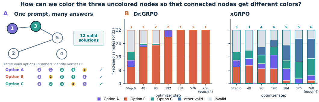
Figure 1: Mode-collapse example. (A) One prompt has 12 valid colorings; three are shown. (B) Four fixed-seed K = 8 draws from matched Qwen2.5-0.5B-Instruct trajectories; color denotes an executed correct mode and gray an invalid response. Dr.GRPO reaches 32/32 correct but contracts to one mode; xGRPO retains six. Accuracy rises while the marginal value of sampling collapses.
