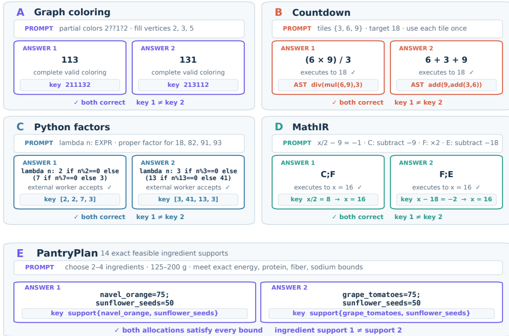
Figure 2: Two verified modes for one prompt in each MODEBENCH domain. Every answer appears inside its own box; the line beneath is the canonical key produced by the same execution that accepted it. Graph answers complete 2 ? ? 1 ? 2; Countdown keys are normalized ASTs; Python keys are executed return vectors; MathIR keys are state trajectories; and PantryPlan keys are ingredient supports. In every panel both answers are correct, but their keys differ. Every panel uses the first row of that domain’s fixed evaluation split. The full prompt behind every panel is in Appendix C.
