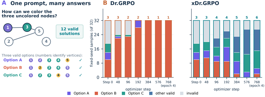
Figure 1: Mode-collapse example. (A) The prompt has 12 valid solutions; three are shown as Options A–C. Numbers inside circles identify vertices, while circle fill denotes assigned color. (B) Separate Dr.GRPO and xDr.GRPO facets show matched Qwen2.5-0.5B-Instruct trajectories (seed 43), never paired bars on one axis. Each bar pools four fixed-seed, eight-sample draws: colored segments are correct modes, gray is invalid output, and the number above each bar is the observed correct-mode count. The x-axis reports optimizer steps and stops at step 768, the end of epoch 4; no epoch-5 checkpoint is shown. Dr.GRPO reaches 32/32 correct but collapses to one mode by step 384 and remains there, while xDr.GRPO retains six modes at step 768. Aggregate results are in Table 3 and Figure 2.
